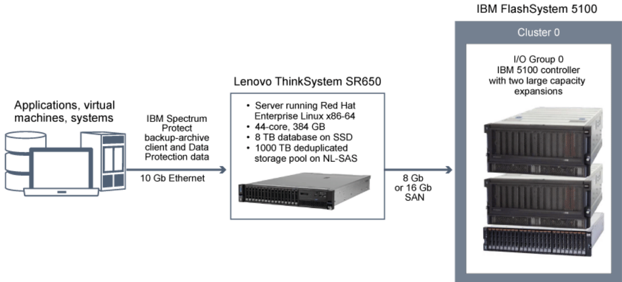
Figure 4. Logical layout for a large system
