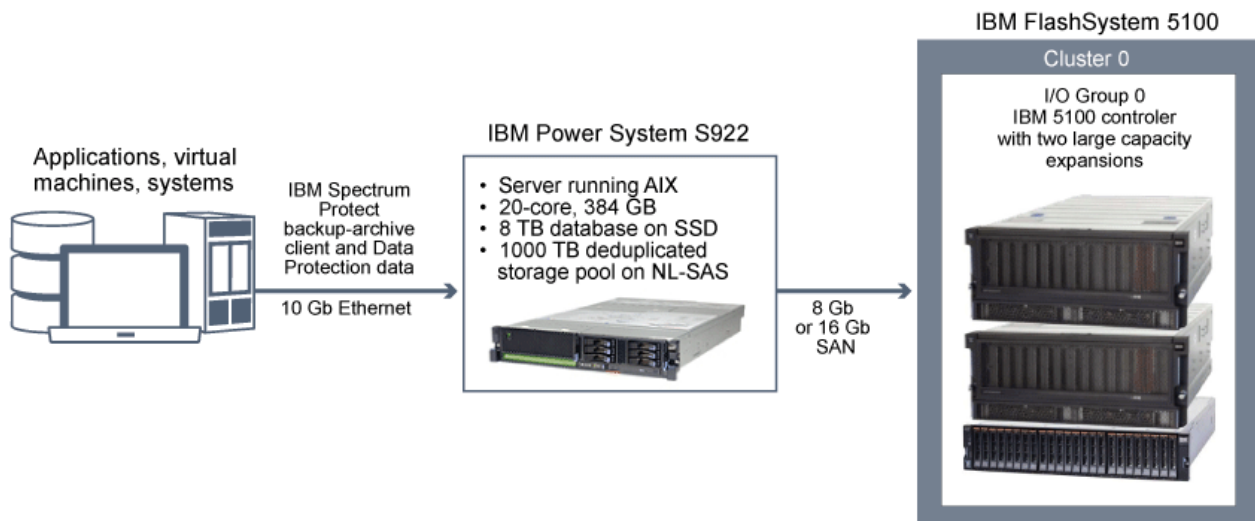
Figure 4. Logical layout for a large system
