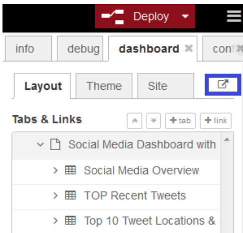
Figure 21. Node-RED dashboard layout panel and URL
