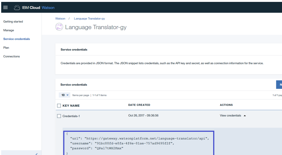
Figure 14. IBM Watson Language Translator service credentials
