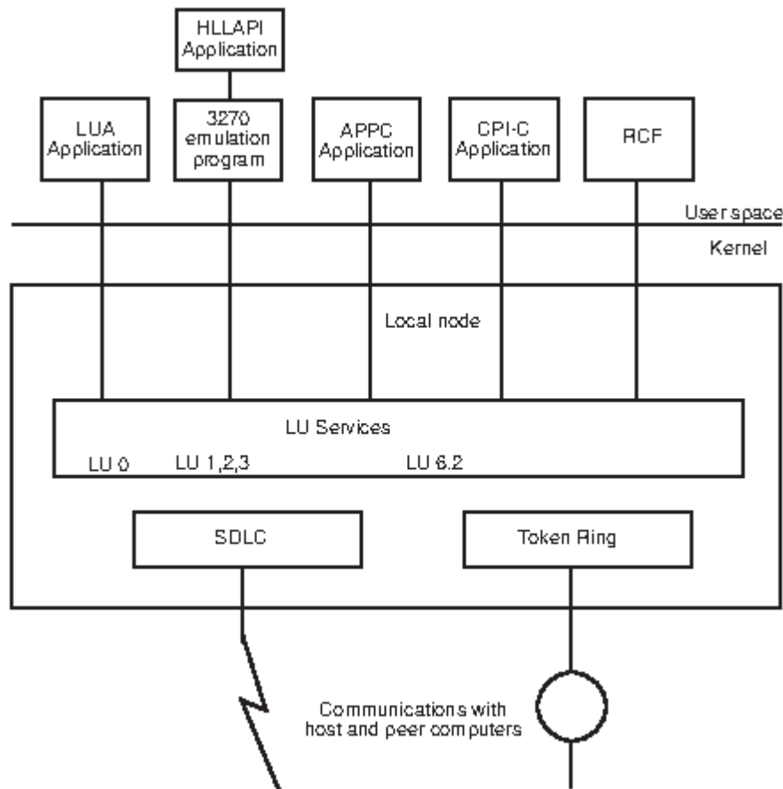
Figure 1. CS/AIX Components
