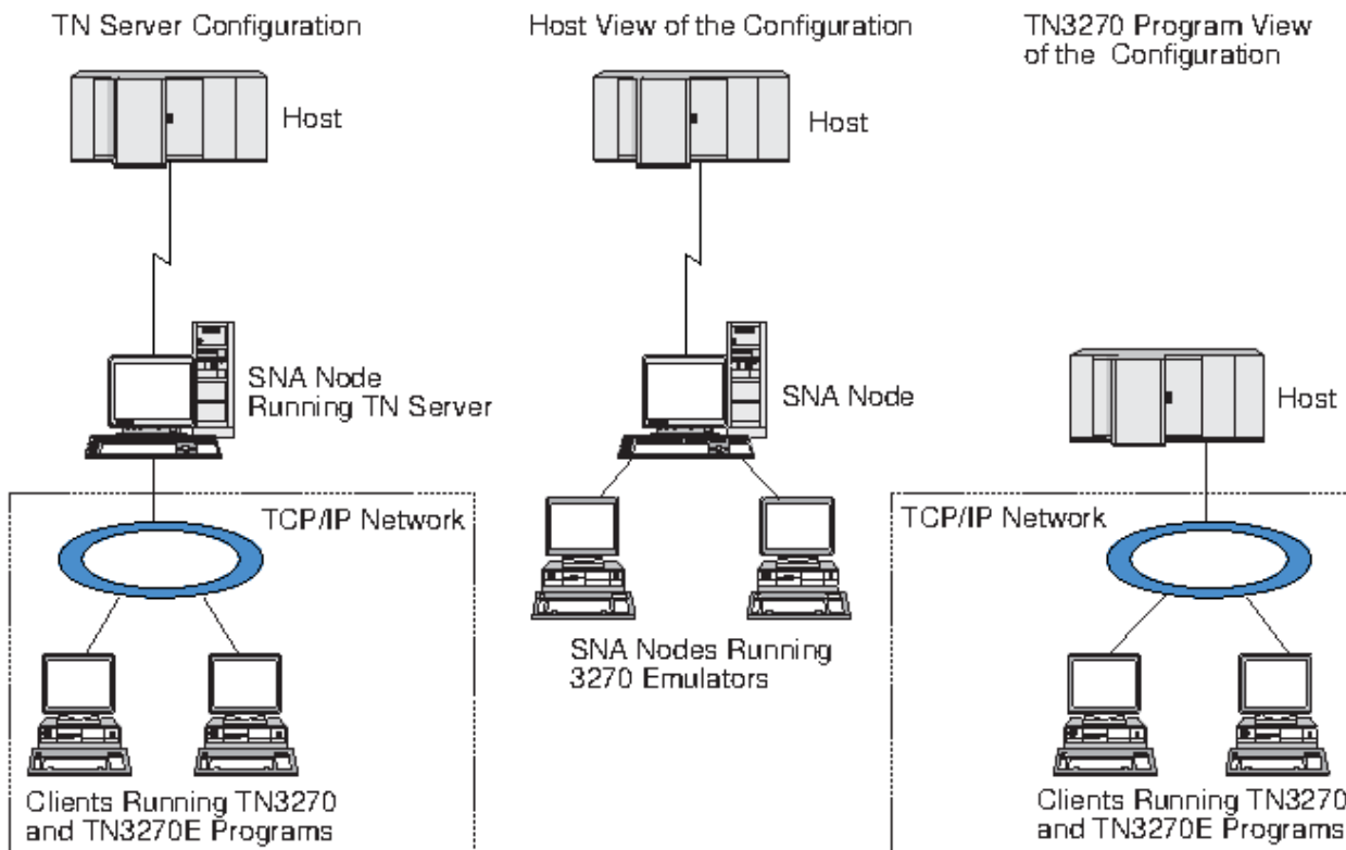
Figure 11. TN Server
