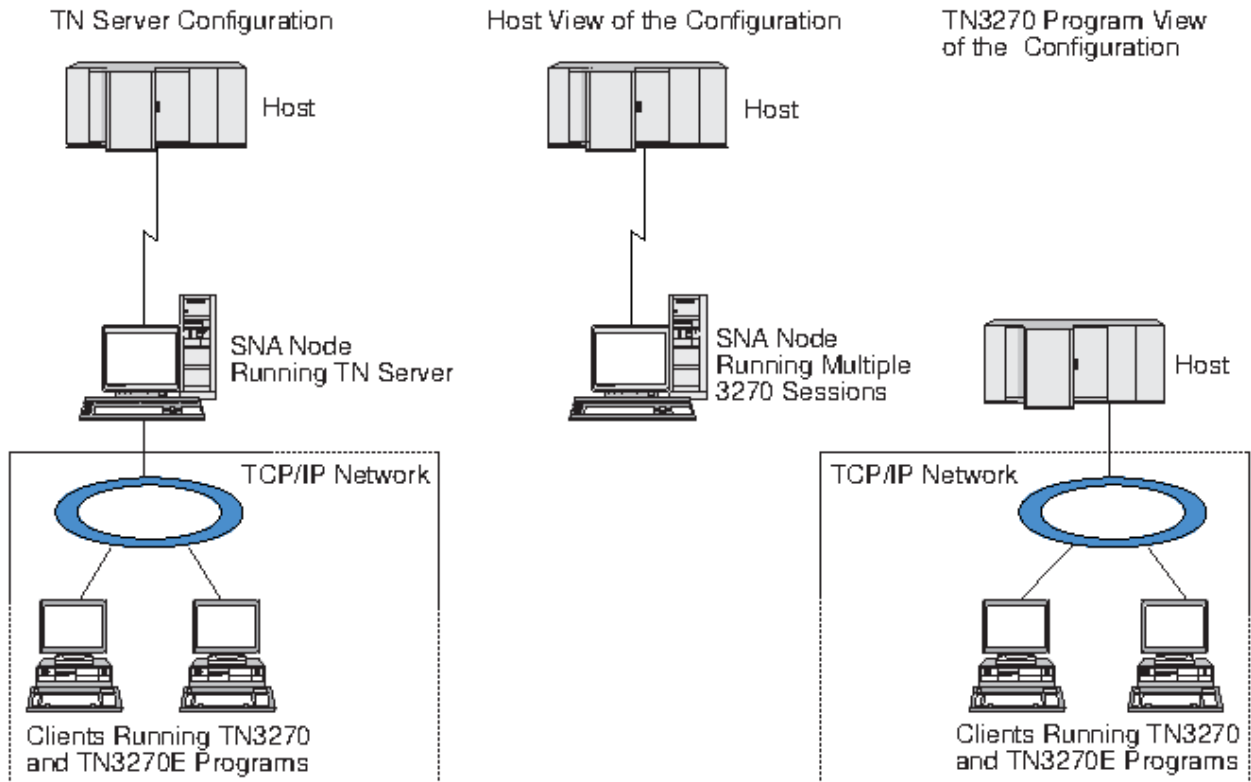
Figure 3. TN Server
