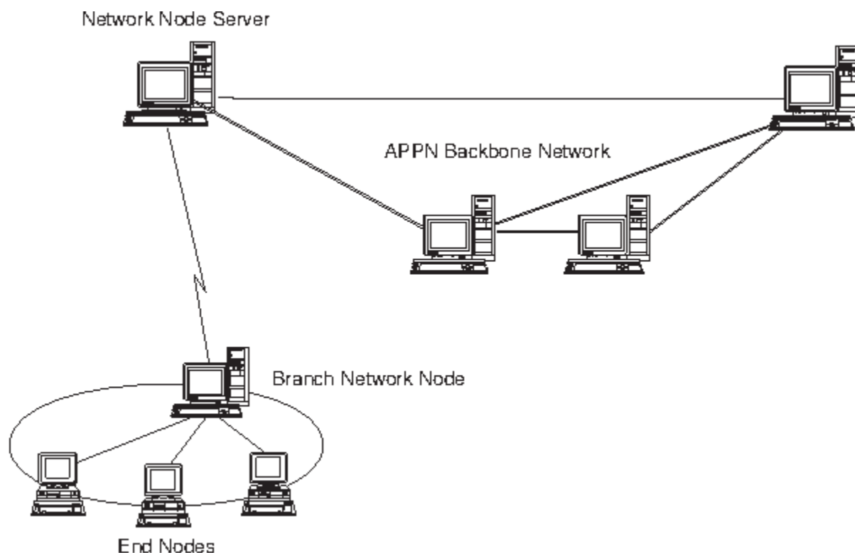
Figure 2. Branch Extender
