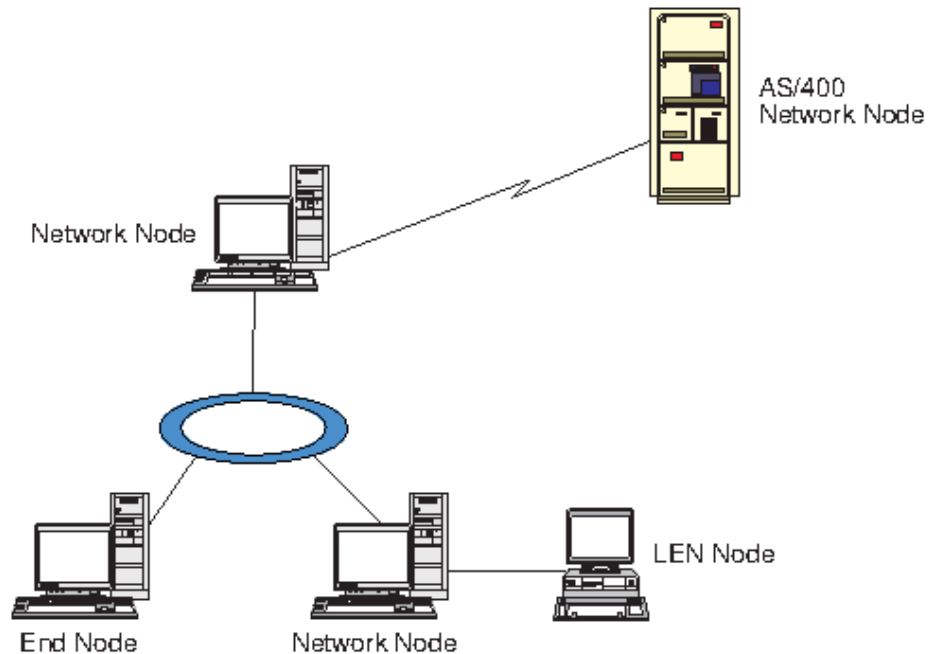
Figure 7. CS Linux Nodes in an APPN Network
