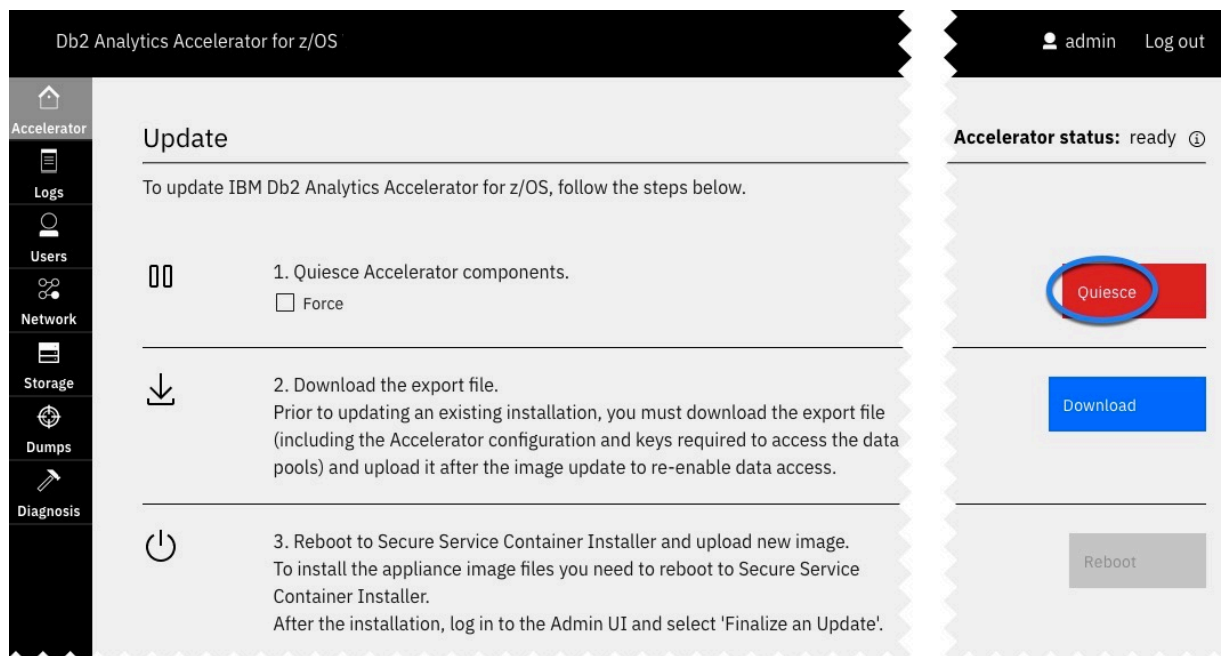
Figure 57. The Update page
