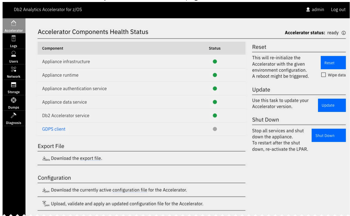
Figure 56. The Accelerator Components Health Status page
