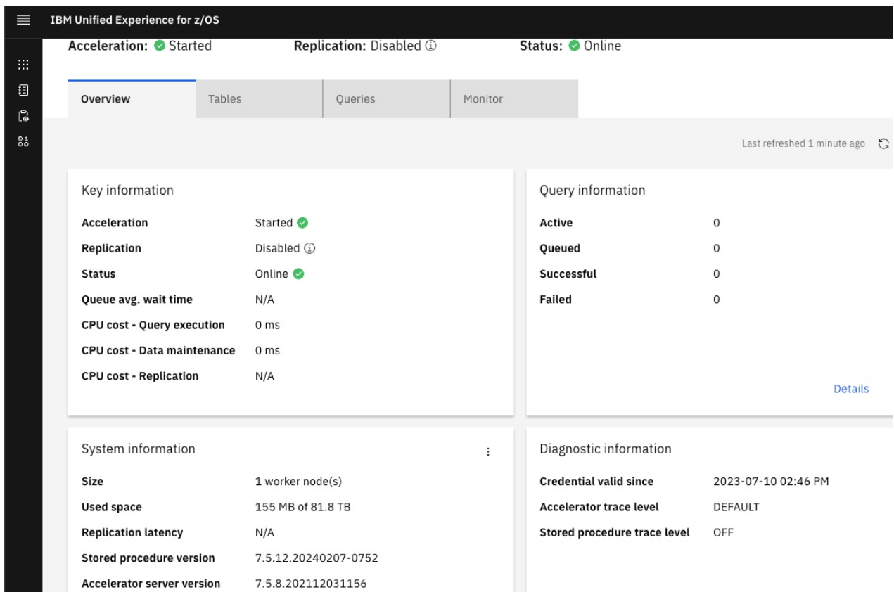
Figure 14. Accelerator details page in IBM Unified Experience for z/OS
