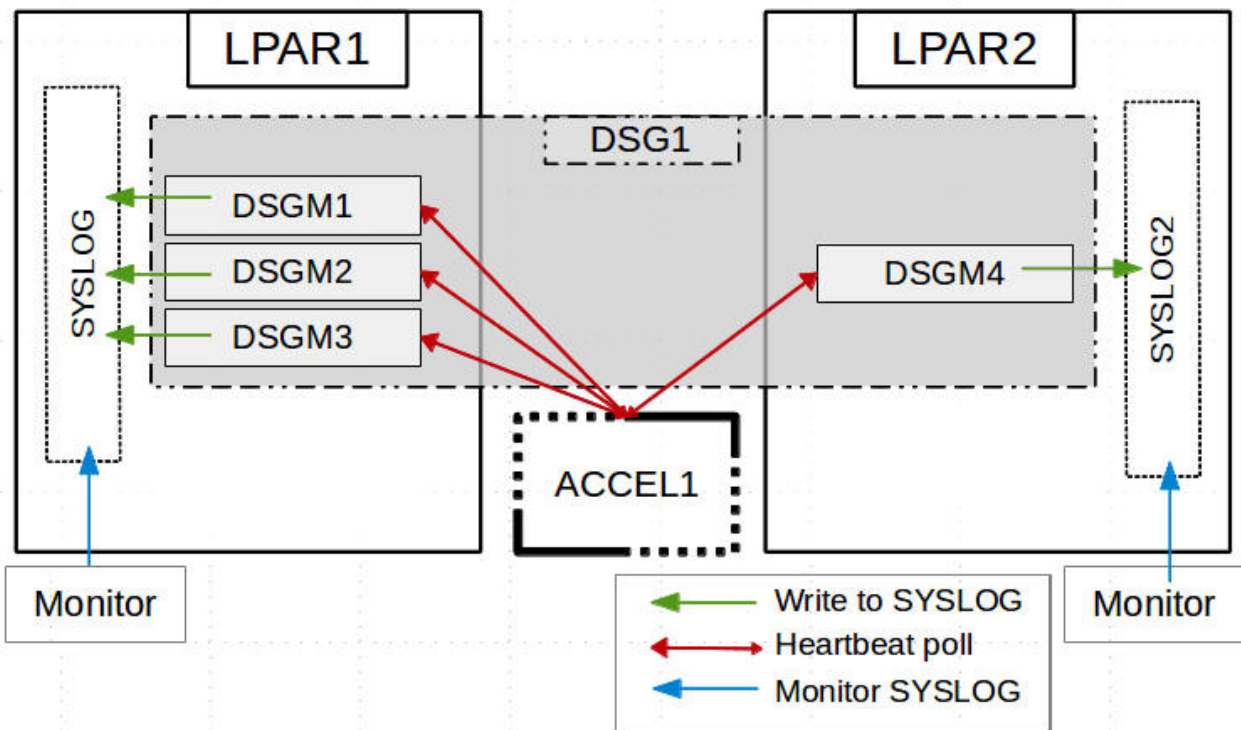
Figure 24. Members in two different LPARs
