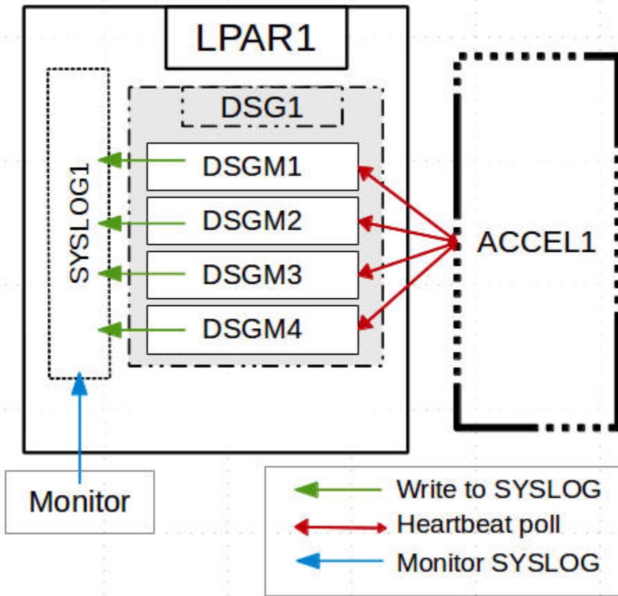
Figure 23. All members in the same LPAR
