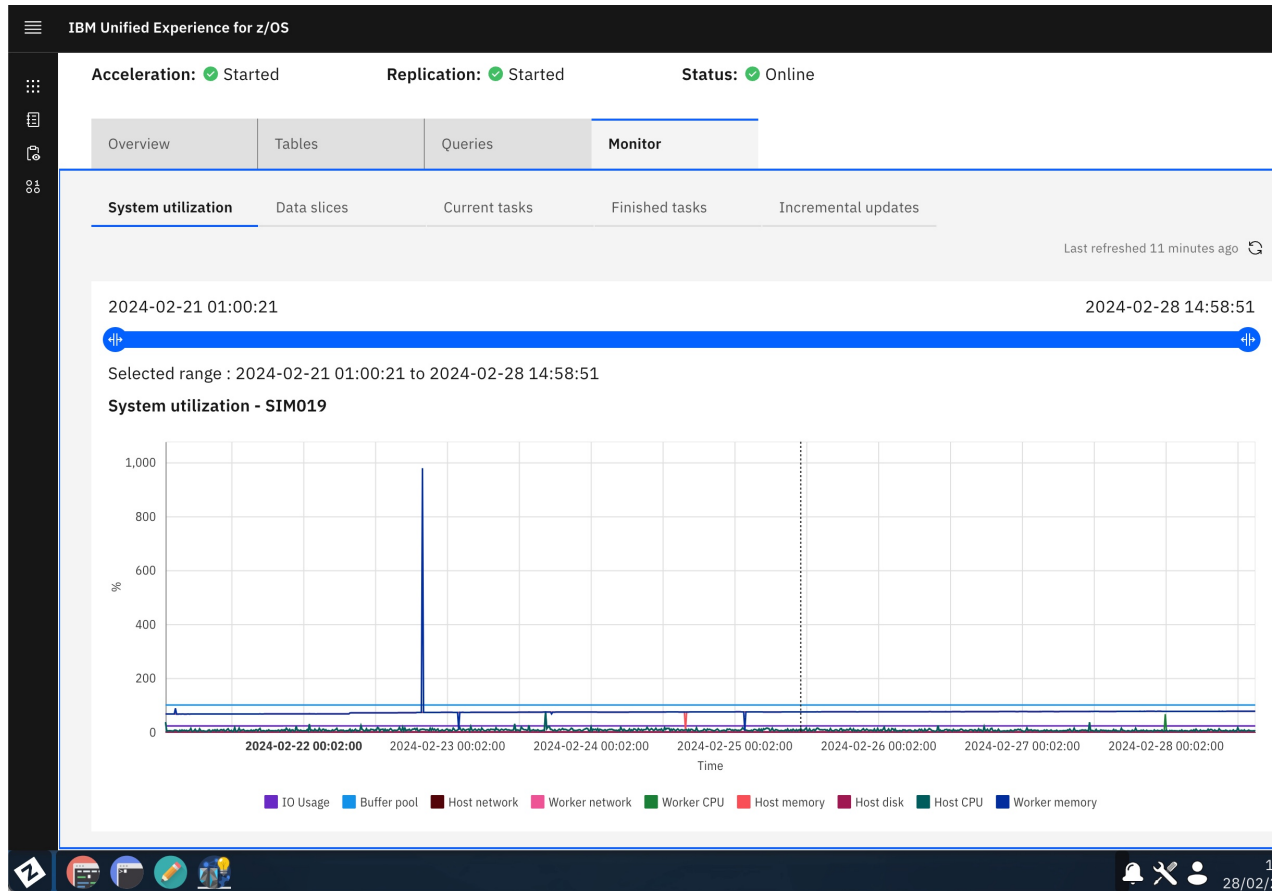
Figure 16. The system utilization graph on the Monitor tab
