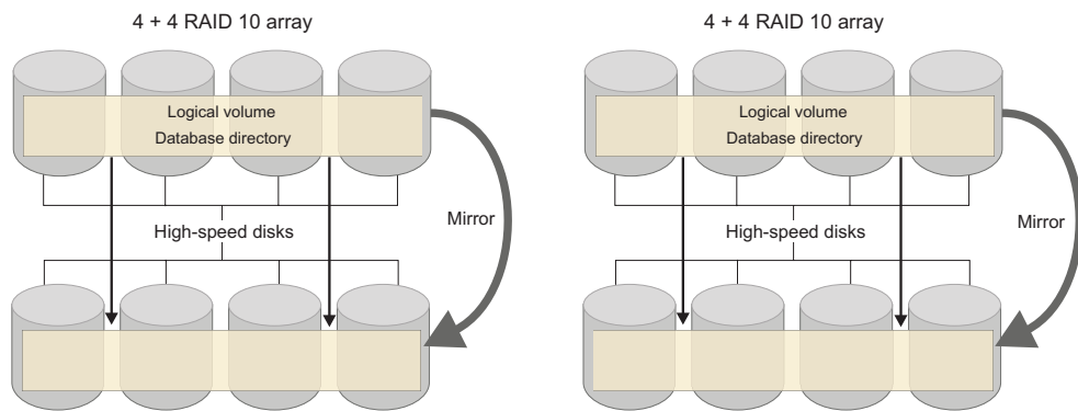
Figure 25. Database layout that uses 16 disks in two RAID 10 arrays
