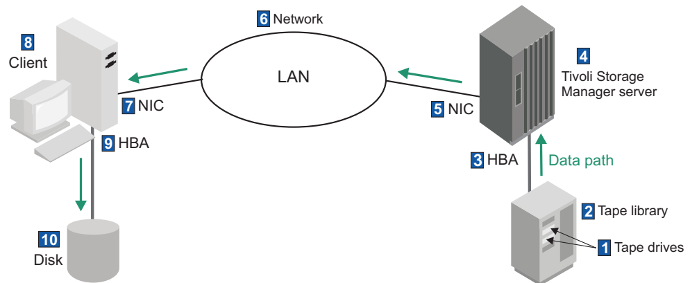
Figure 18. Data flow for restore operations for database applications
