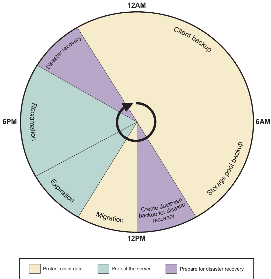
Figure 21. Daily schedule of Tivoli Storage Manager operations
