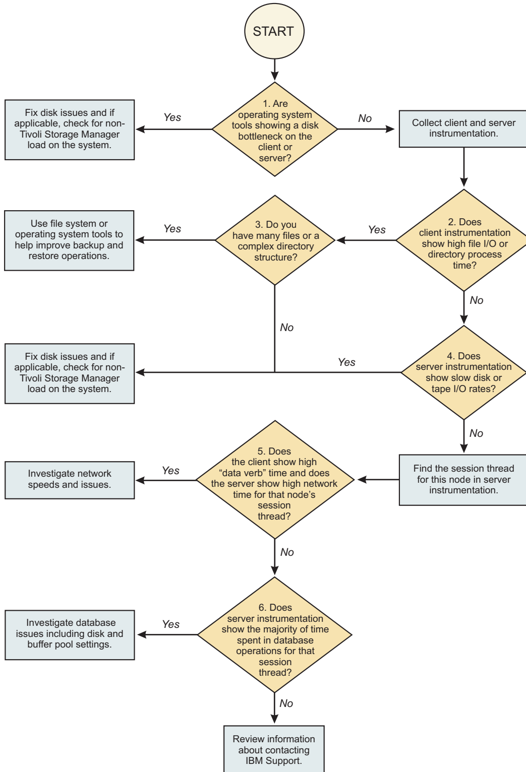
Figure 4. Flowchart to diagnose backup and restore performance. Use this chart with Table 3 on page 57.
