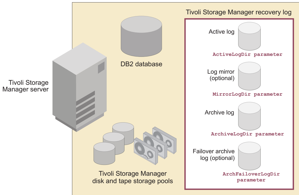
Figure 19. Components of the Tivoli Storage Manager database and recovery log
