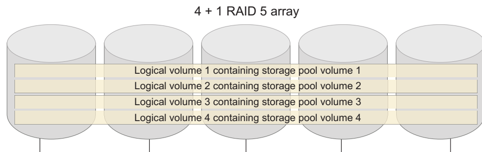
Figure 27. Storage pool layout with 4 + 1 RAID 5
