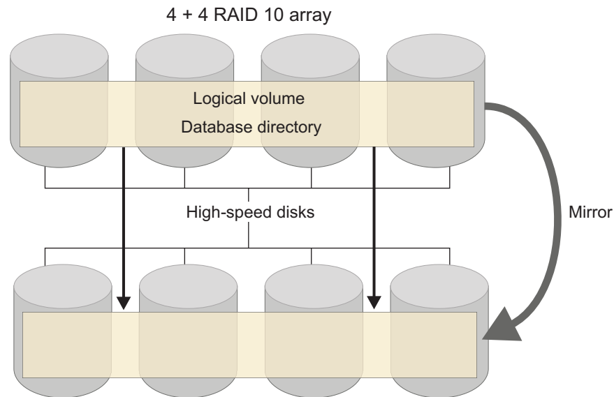
Figure 24. Database layout that uses eight disks in a RAID 10 array
