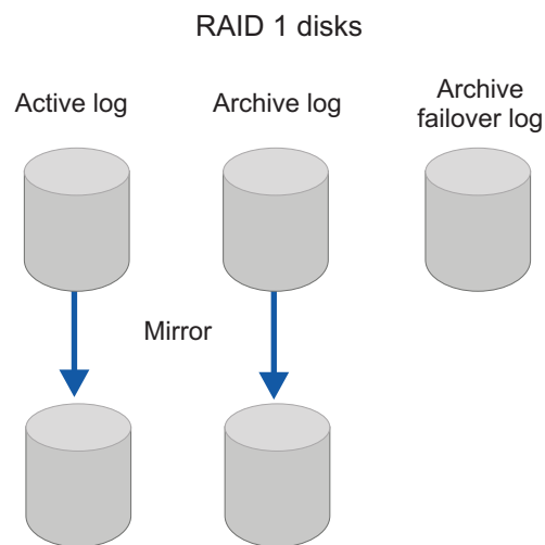
Figure 26. Logs layout with RAID 1
