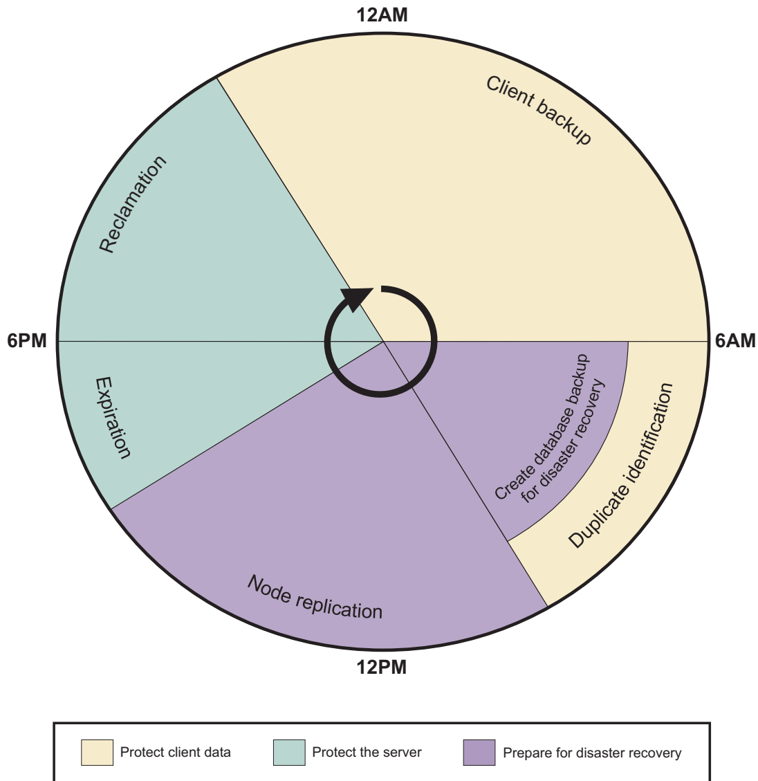
Figure 22. Daily schedule when data deduplication and node replication are used
