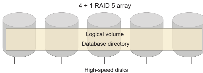
Figure 23. Database layout for a small server
