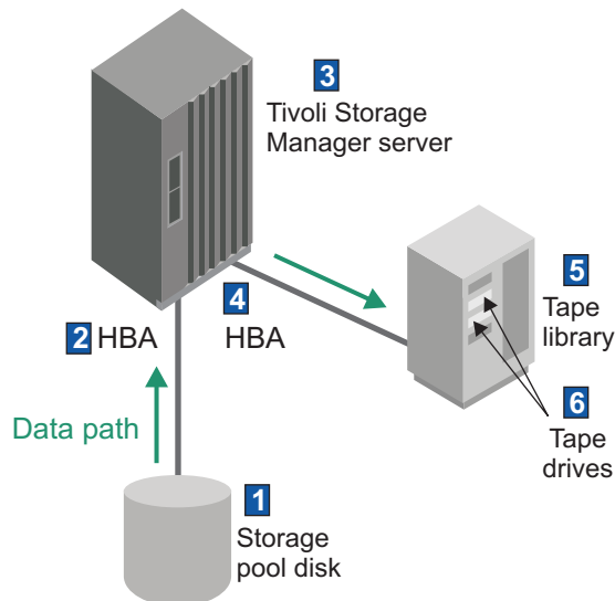
Figure 16. Data flow for migration operations
