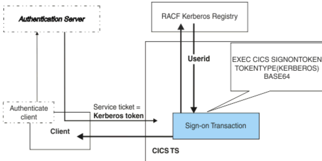
Figure 32. Flow of requests between the Client terminal emulator, the authentication server, and CICS TS
