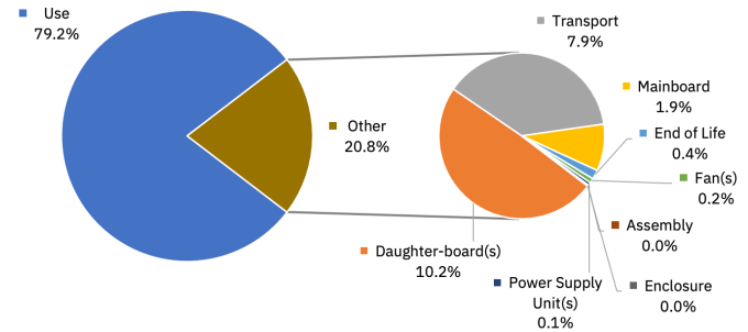
Figure 3: Carbon footprint impact by phase for the IBM z16™ single frame PCIe+ I/O drawer typical product configuration listed in Table 3 using the PAIA model; 79.2% occurs in the use phase and the remaining 20.8% is broken out.
