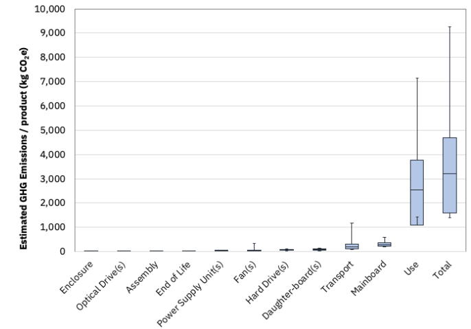
Figure 6: Uncertainty in the PCF estimate for the IBM z16™ single frame Support Element typical product configuration listed in Table 4; the estimate has a total mean of 3,000 ± 2,000 kg CO 2 e over a use period of 5 years.
