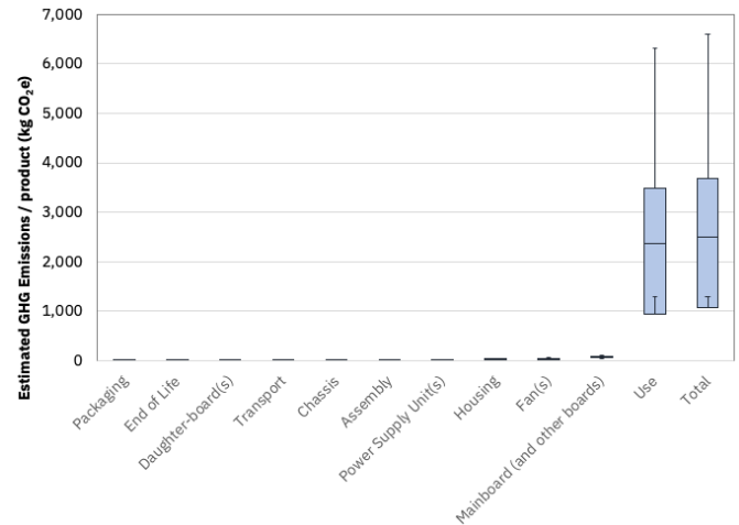
Figure 8: Uncertainty in the PCF estimate for the IBM z16™ single frame 24-port Ethernet Switch typical product configuration listed in Table 5; the estimate has a total mean of 3,000 ± 2,000 kg CO 2 e over a use period of 5 years.
