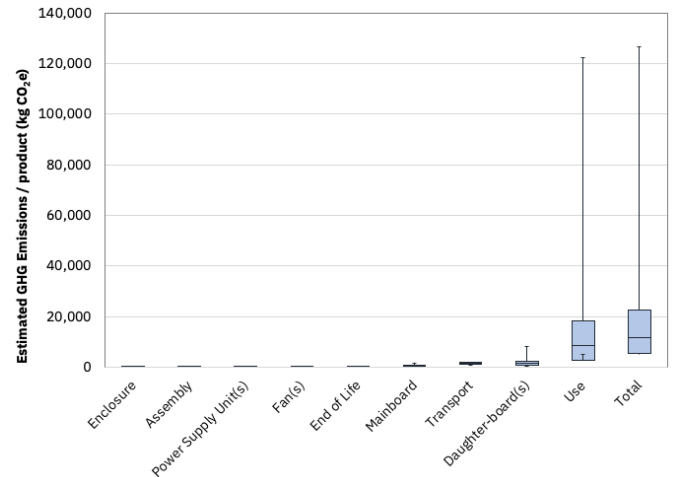
Figure 4: Uncertainty in the PCF estimate for the IBM z16™ single frame PCIe+ I/O drawer typical product configuration listed in Table 3; the estimate has a total mean of 18,000 ± 20,000 kg CO 2 e over a use period of 5 years.
