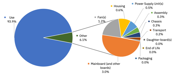
Figure 7: Carbon footprint impact by phase for the IBM z16™ single frame 24-port Ethernet Switch product configuration listed in Table 5 using the PAIA model; 93.9% occurs in the use phase and the remaining 6.1% is broken out.
