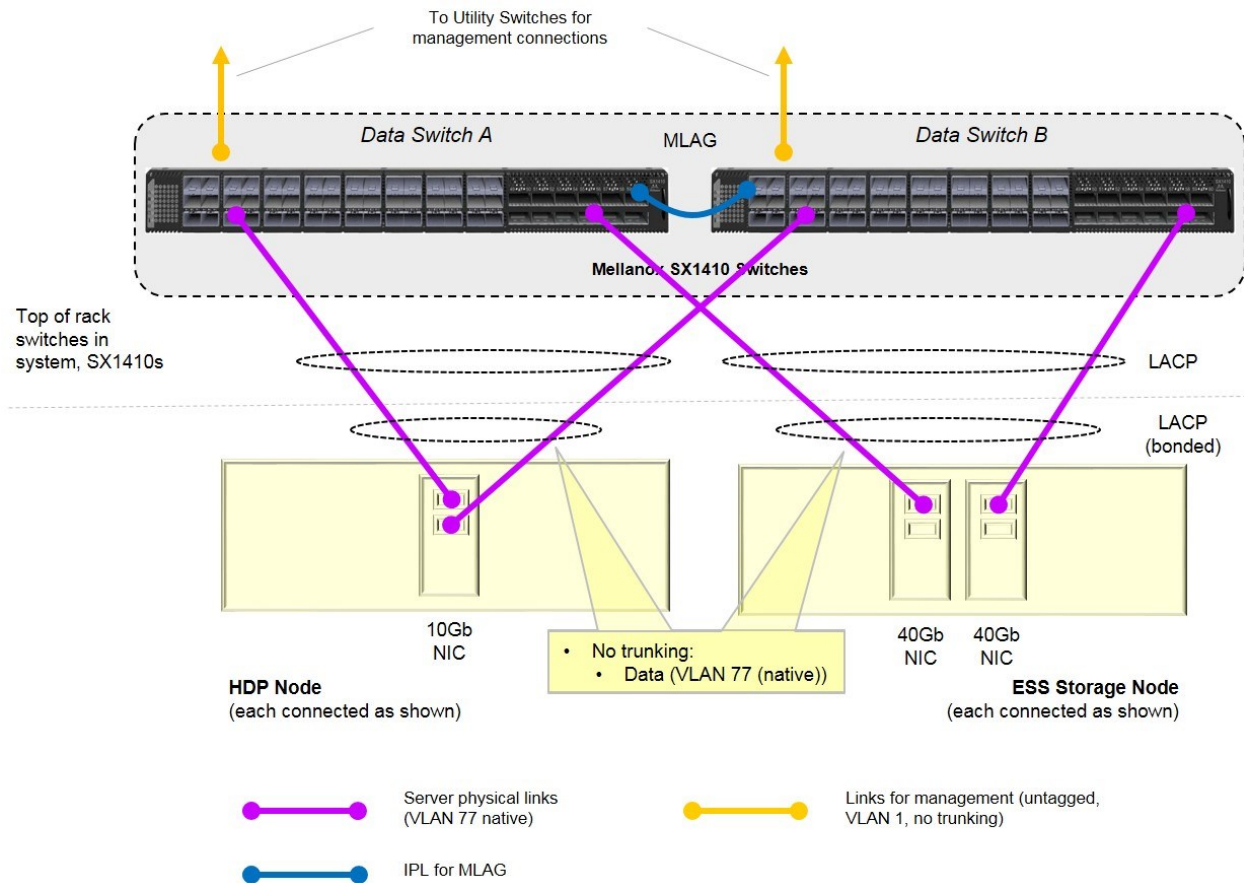
Figure 22. Data Switch Cabling - Physical Schematic View
