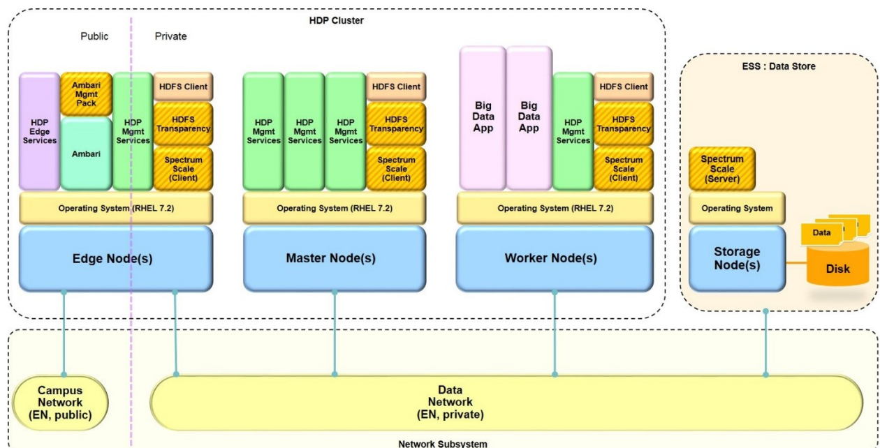
Figure 9. Architecture – Platform View – Node Types and Hosting Focus
