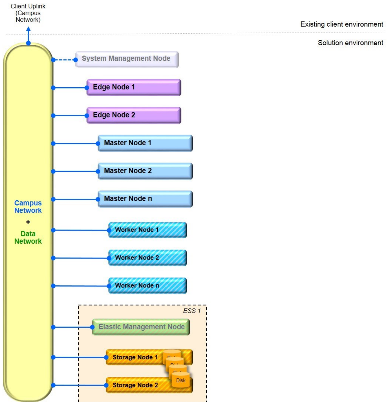
Figure 56. Flat Network
