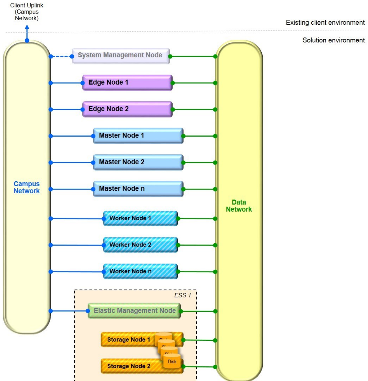
Figure 55. Dual-Homed Network
