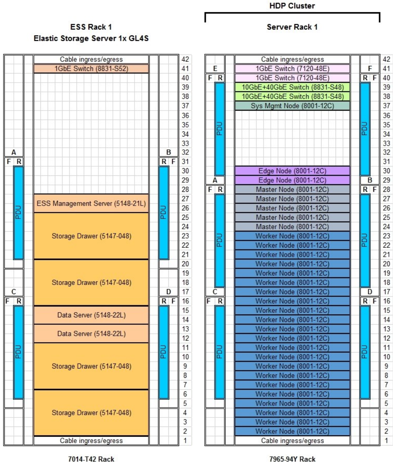
Figure 43. Physical Rack Layout
