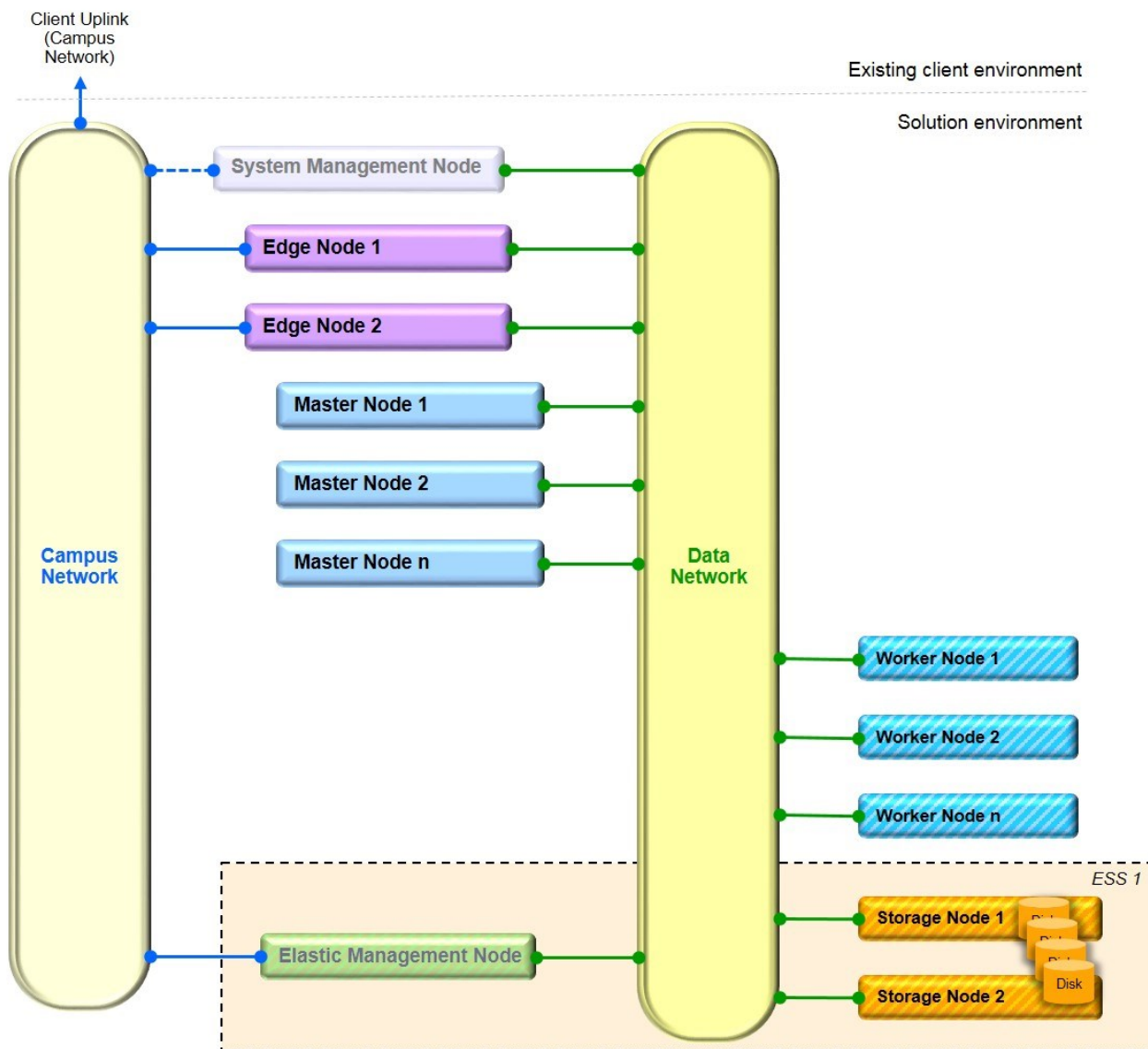
Figure 11. Partial-Homed Network
