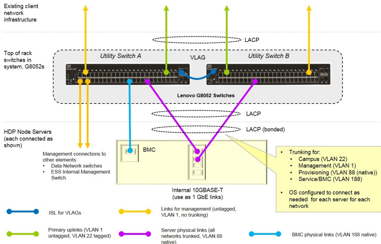
Figure 21. Utility Switch Cabling - Physical Schematic View
