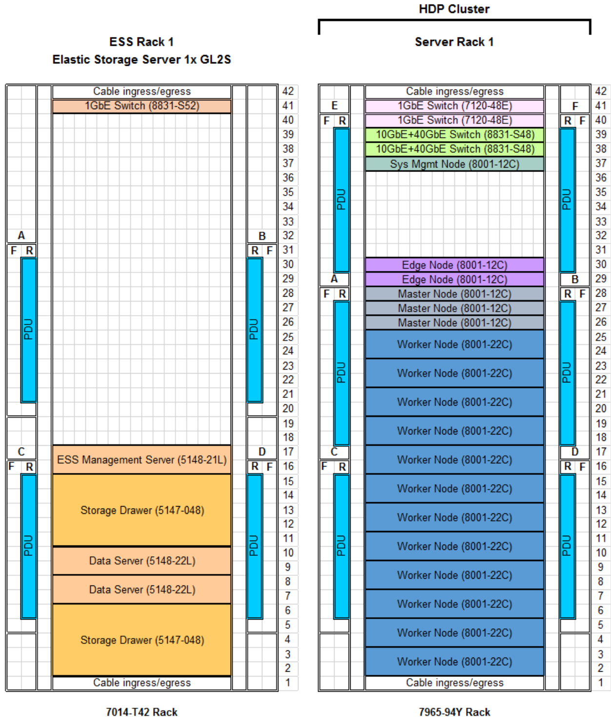
Figure 25. Physical Rack Layout
