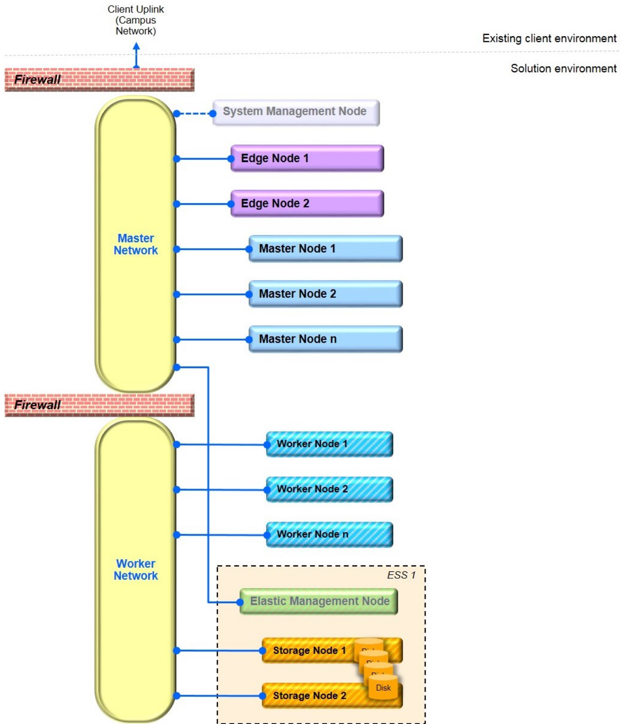
Figure 57. DMZ Network
