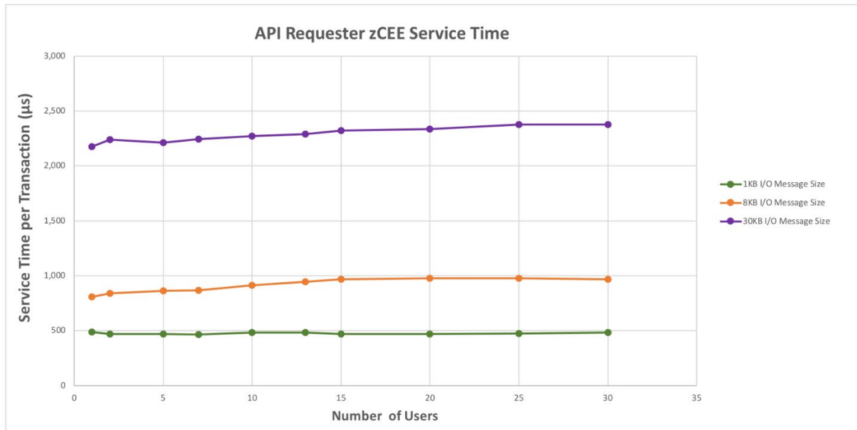
Figure 35 shows the z/OS Connect Service Time per transaction for 10 users.
