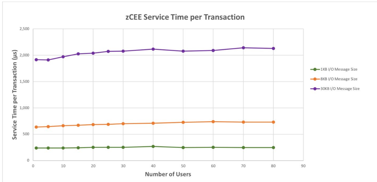
Figure 21 shows the z/OS Connect IMS SP Service Time per transaction for 30 users.
