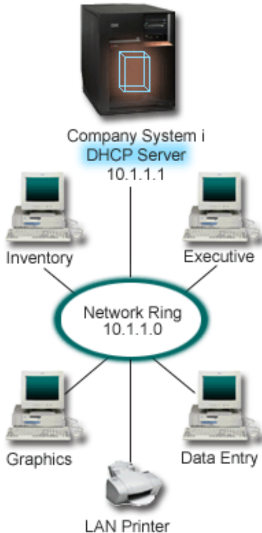
Figure 2. Simple LAN setup for System i model
