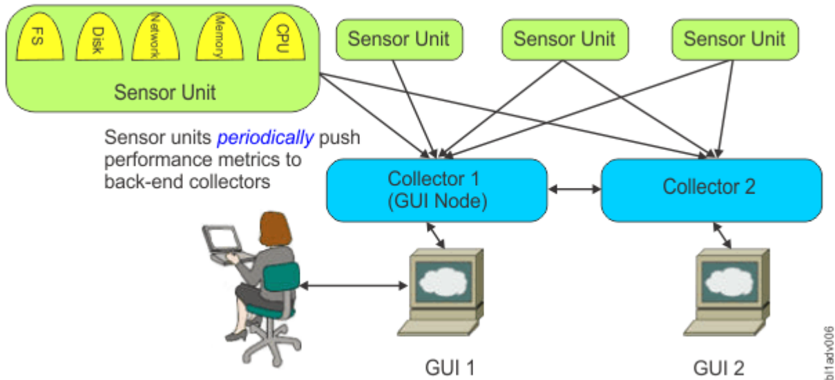
Figure 2. Performance monitoring configuration for GUI
