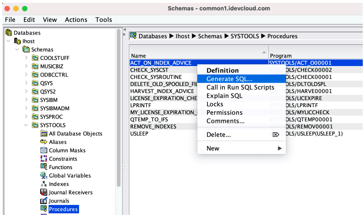
Figure 2. Launching Generate SQL from IBM i Access Client Solutions (ACS):
