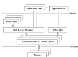
Figure 44. Multiple user and multiple adapter configuration
