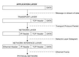
Figure 5. Movement of information from sender application to receiver host
