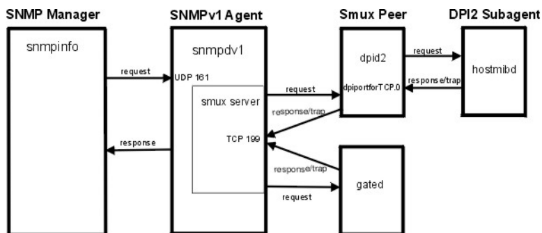
Figure 28. The primary parts of the SNMPv1 architecture
