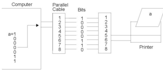
Figure 29. Parallel communications port
