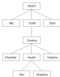
Figure 22. Domain structure of the Internet
