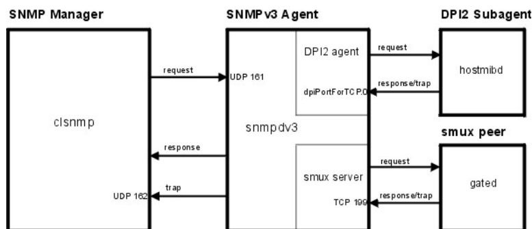
Figure 27. The primary parts of the SNMPv3 architecture
