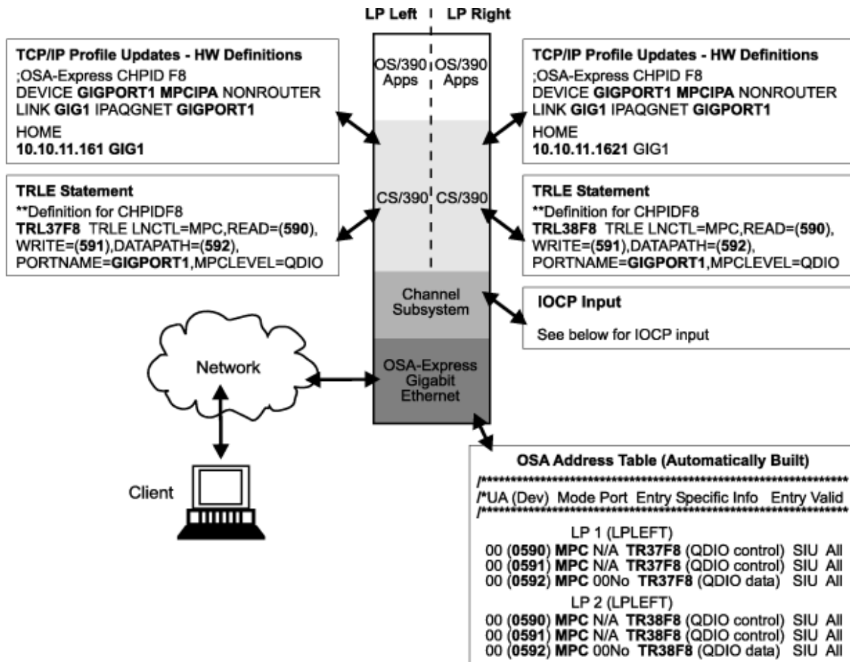
Figure 46. OSA configuration with two logical partitions
