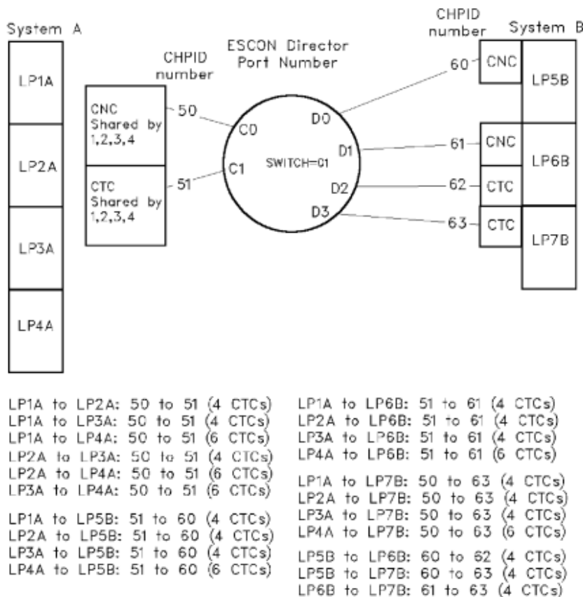
Figure 50. ESCON CTC with shared and unshared channels
