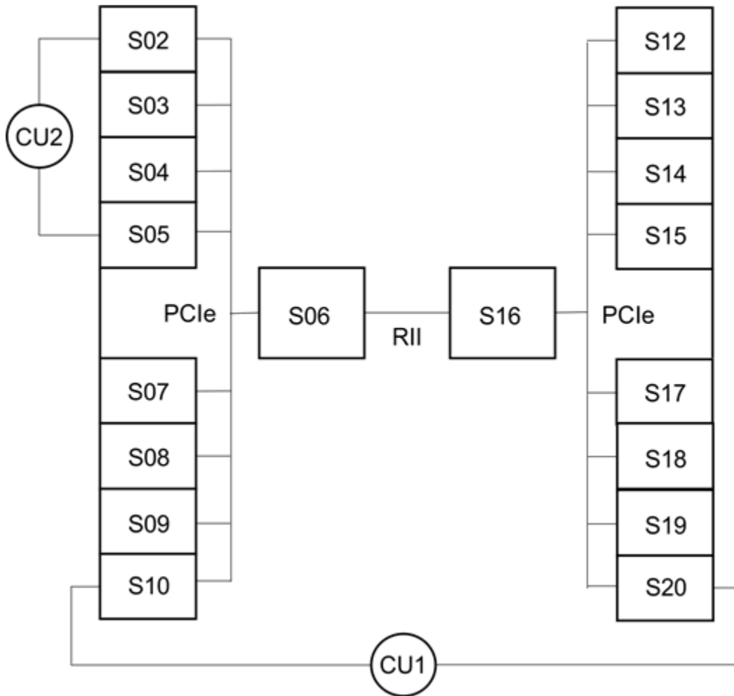
Figure 2. I/O channel path configuration for a representative PCIe I/O drawer in a 8562, 8561, and 3907 model
