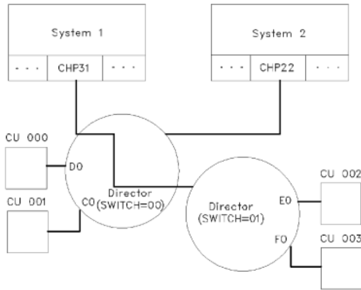
Figure 40. Chained ESCON directors
