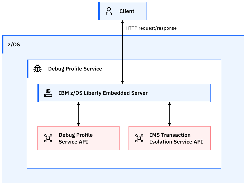
Figure 14. Debug Profile Service
