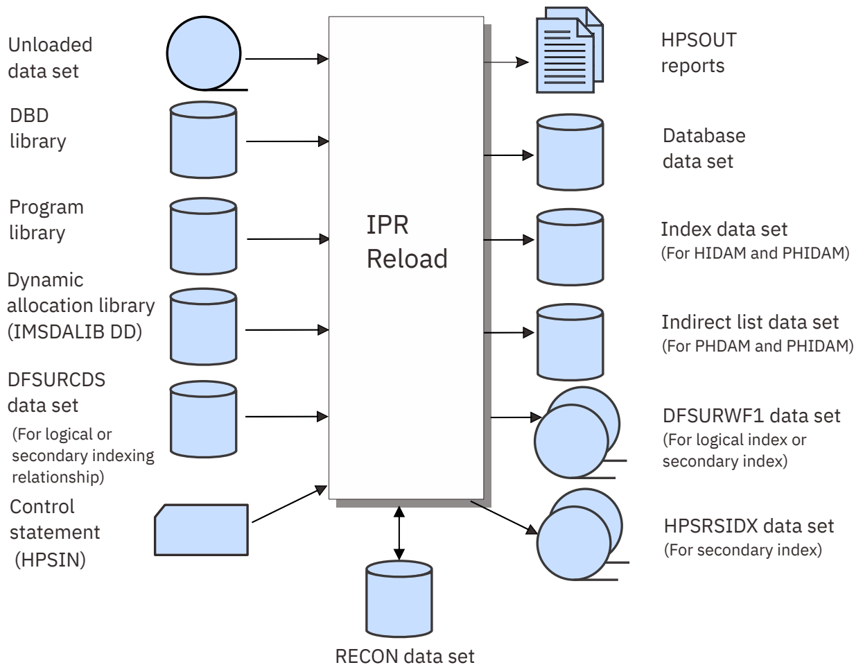
Figure 178. Data flow of the IPR Reload utility
