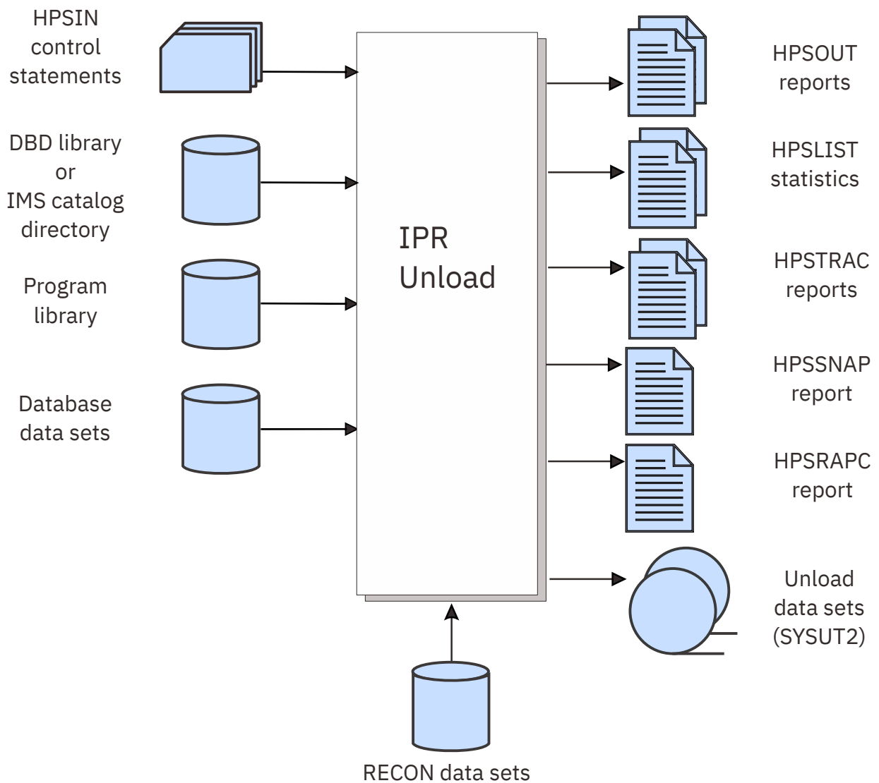
Figure 131. Data flow of the IPR Unload utility
