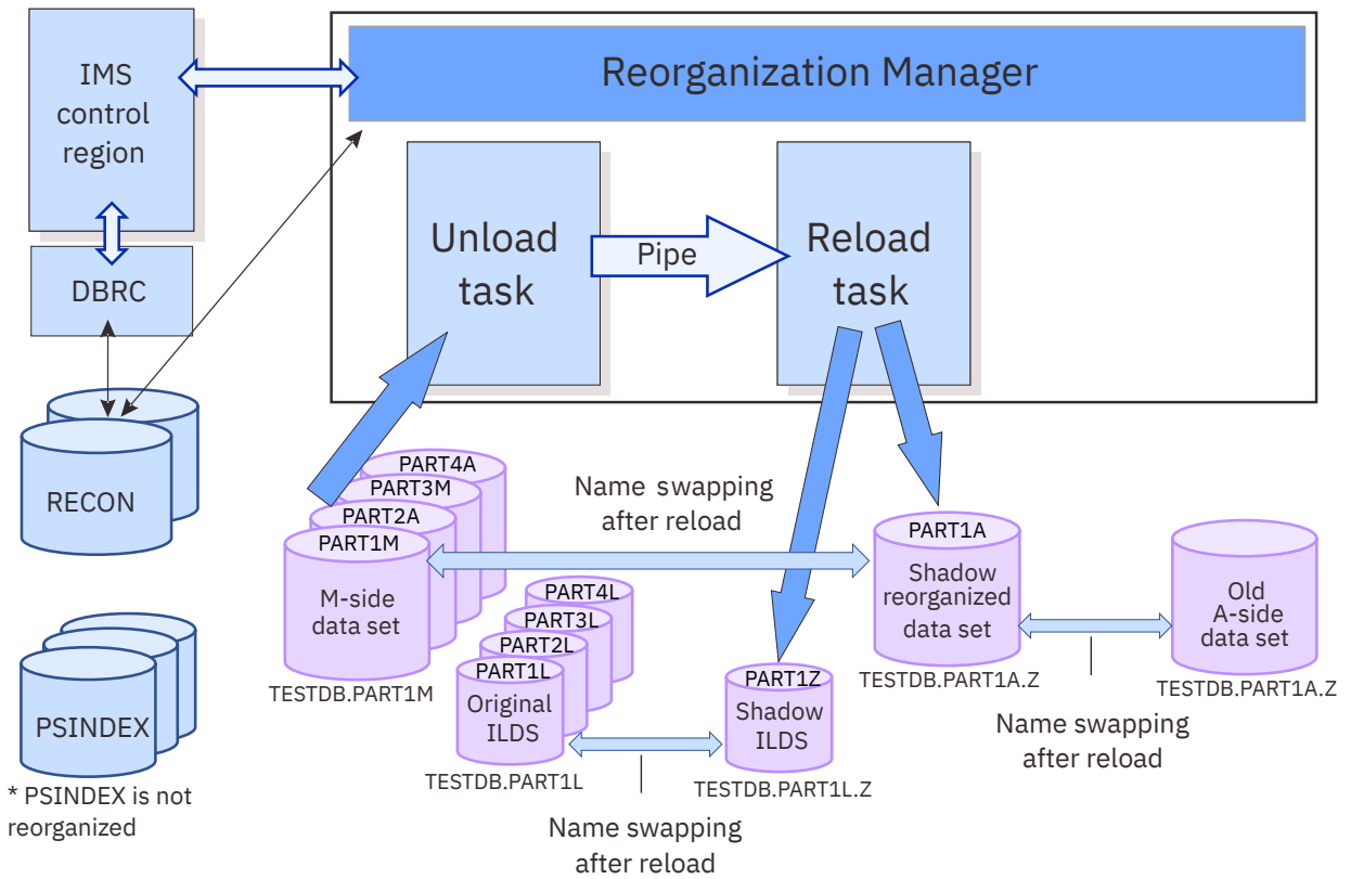
Figure 8. System flow of the Parallel Reorganization Service for PHDAM with PSINDEX (3)
