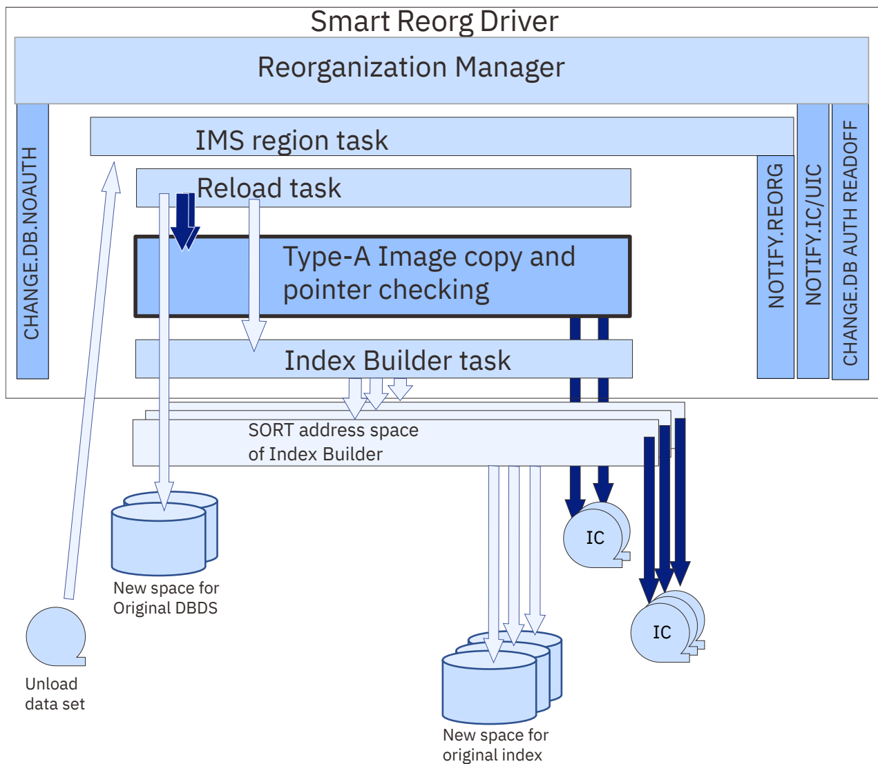
Figure 11. Data and process flow of reloading a database and taking an image copy
