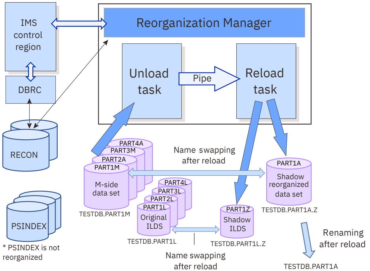
Figure 7. System flow of the Parallel Reorganization Service for PHDAM with PSINDEX (2)
