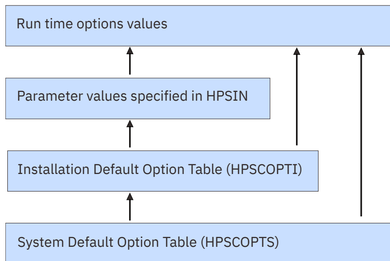
Figure 225. How runtime options are determined
