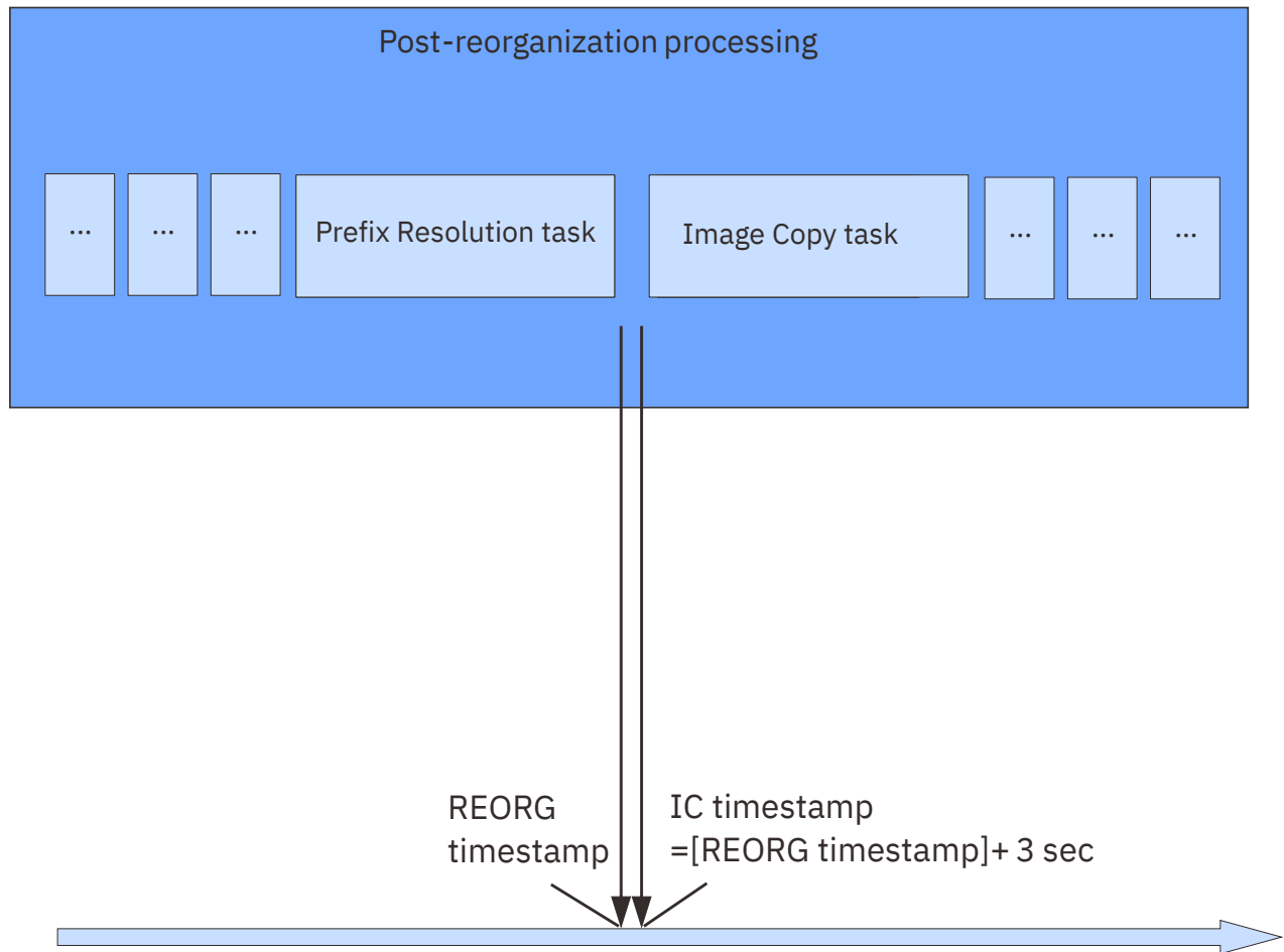
Figure 104. REORG and IC timestamps during Post-reorganization processing
