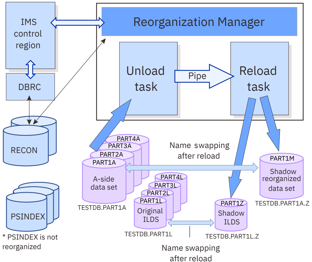
Figure 6. System flow of the Parallel Reorganization Service for PHDAM with PSINDEX (1)
