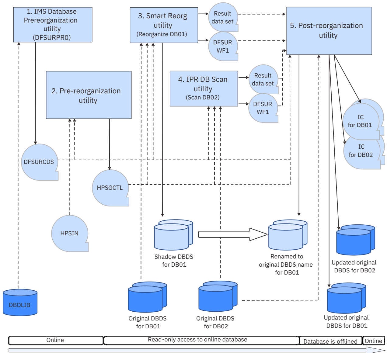
Figure 102. Process flow for reorganizing databases that have external logical relationships
