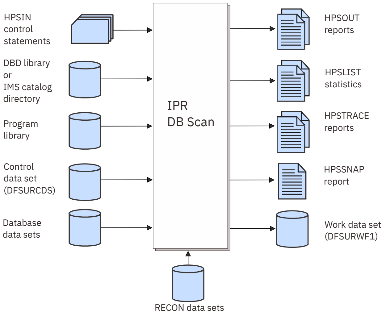
Figure 217. Data flow of the IPR DB Scan utility
