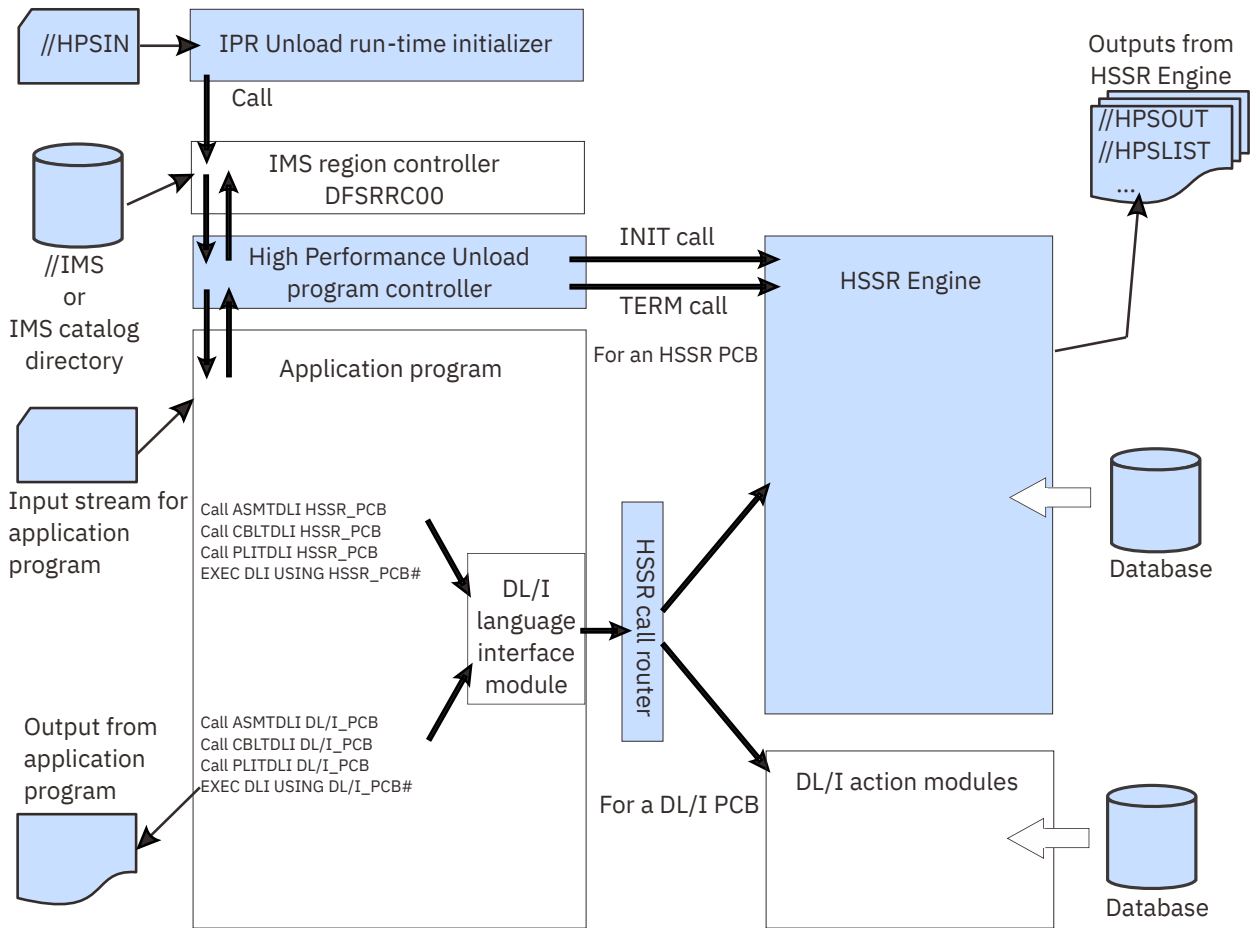
Figure 172. System flow of the API function
