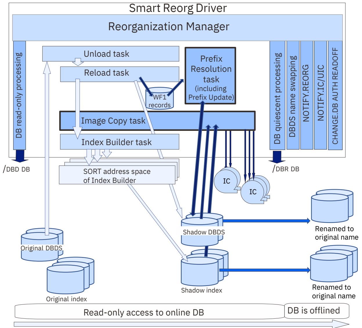
Figure 10. Data and process flow of Type-B Image Copy with Prefix Resolution/Update
