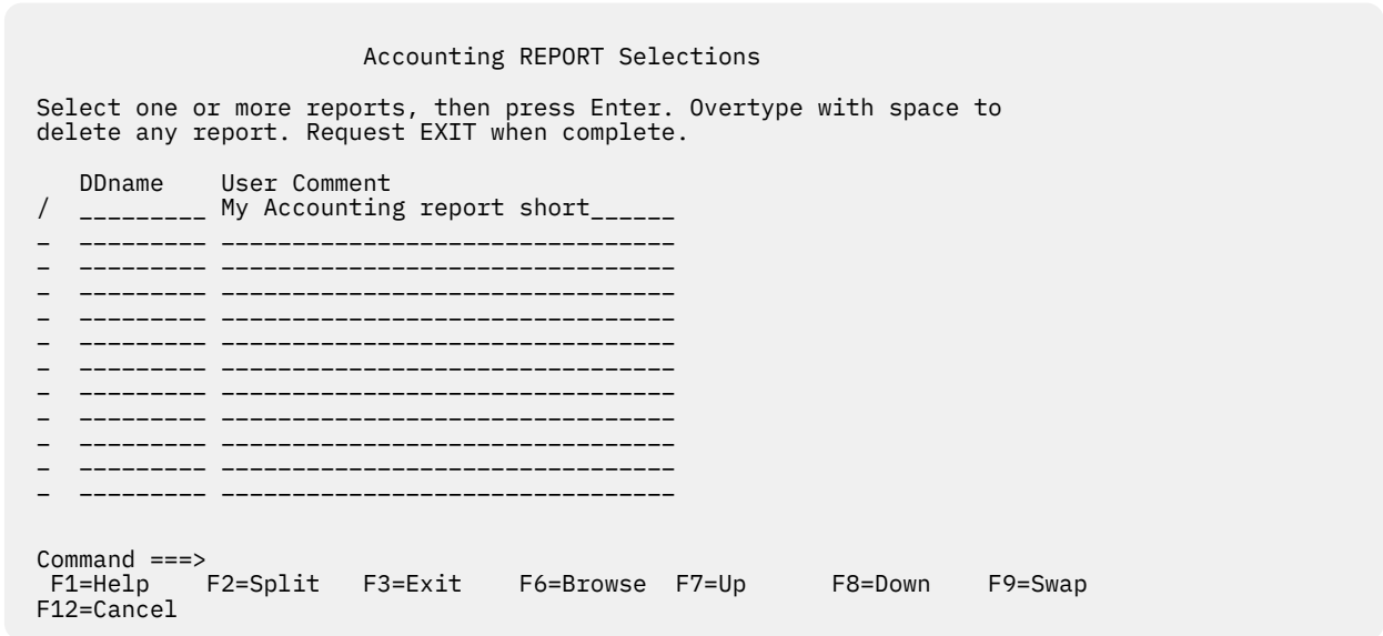
Figure 16. Accounting Report Selections panel
