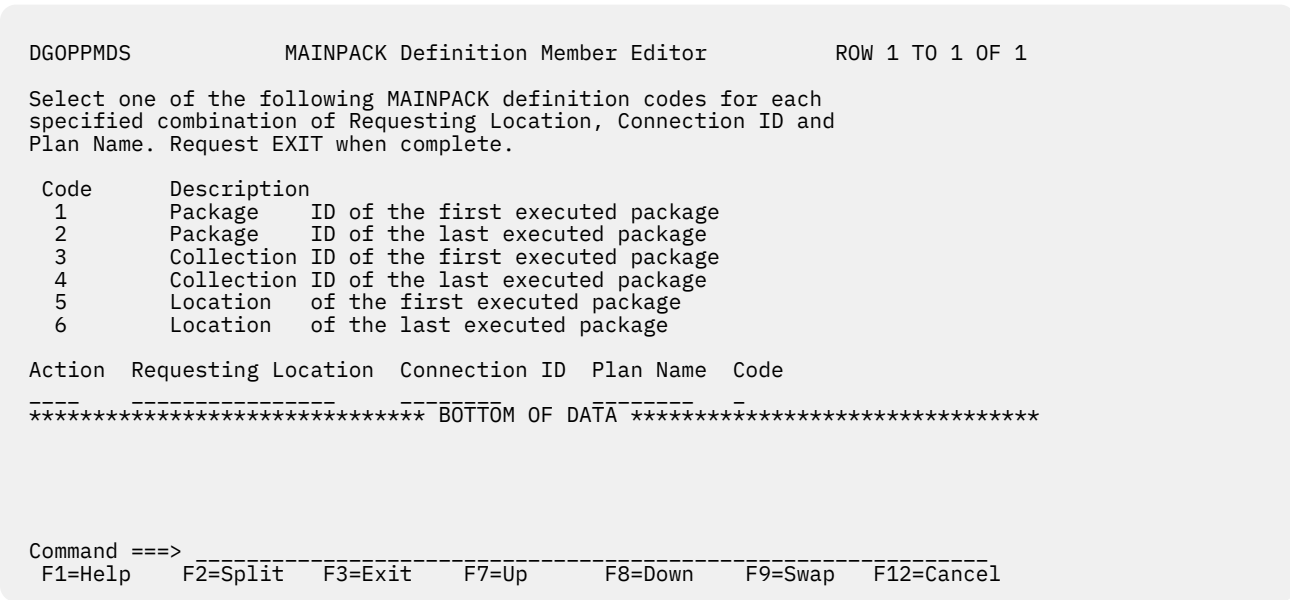
Figure 62. MAINPACK Definition Member Editor panel
