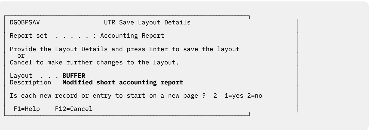
Figure 55. User-Tailored Reporting - saving the layout
