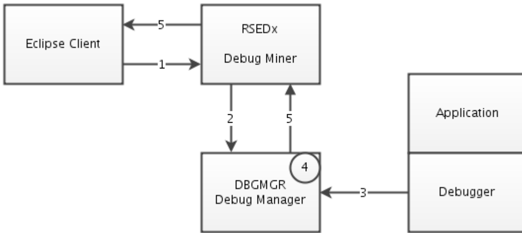
Figure 2. Debug Manager
