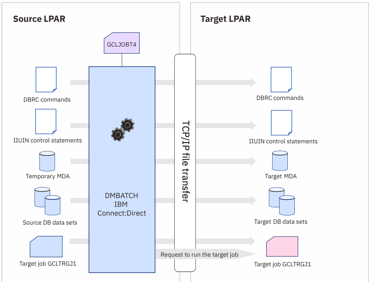
Figure 2. Process flow of the TCP/IP data transfer job
