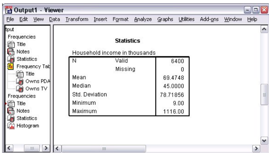
Figure 30. Frequencies Statistics table
