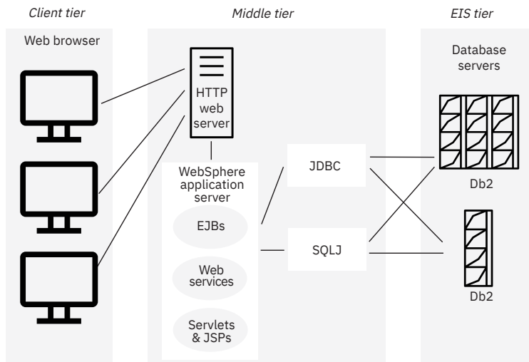
Figure 53. n -tier connectivity with a workstation-based client, two web servers, and different database servers
