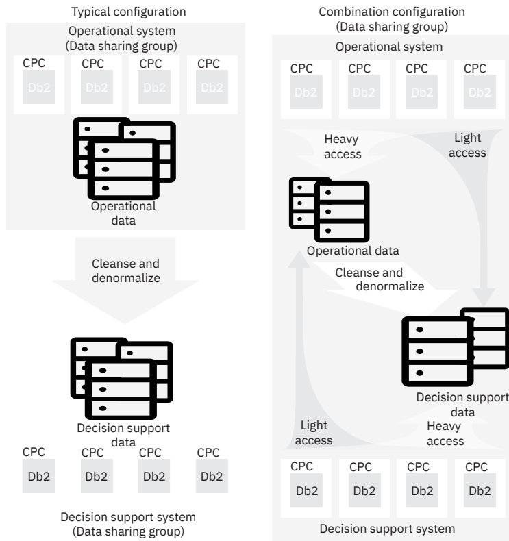
Figure 34. Flexible configurations for decision support
