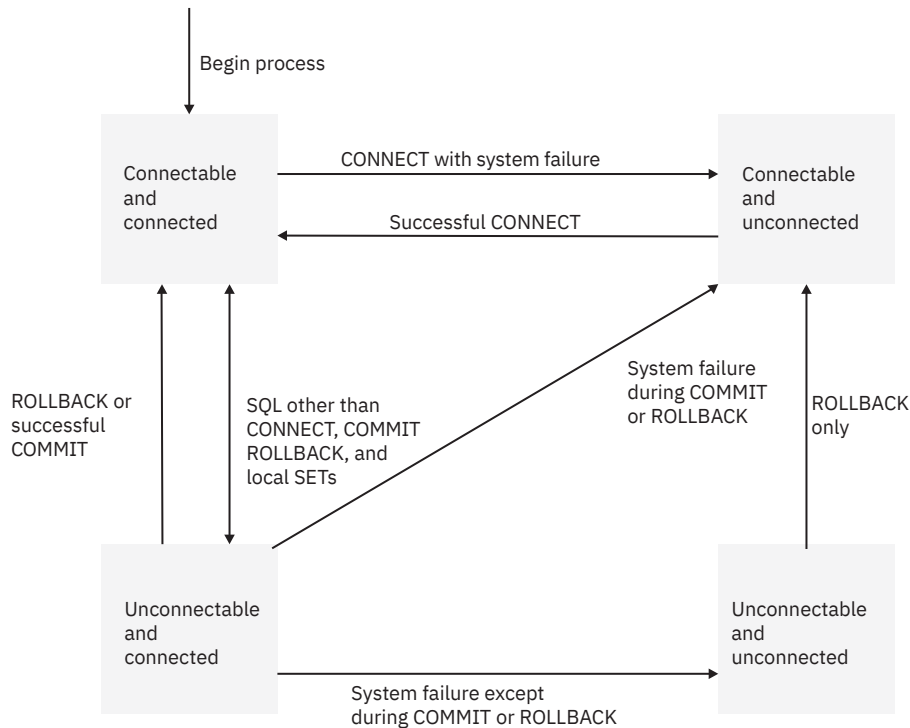
Figure 28. State transitions for an application process connection in a remote unit of work
