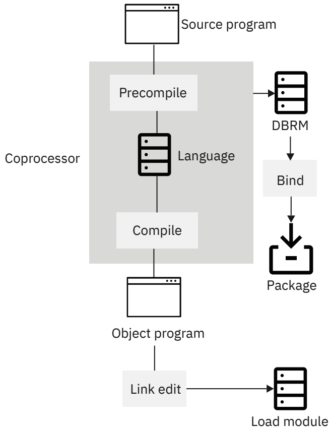
Figure 49. Overview of the program preparation process for applications that contain embedded SQL. The Db2 coprocessor can combine the precompile and compile steps for certain languages.
