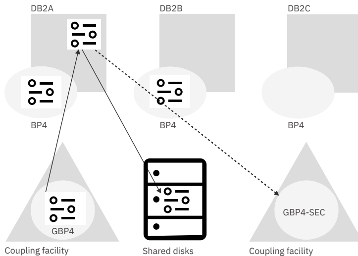
Figure 40. Writing data to disk
