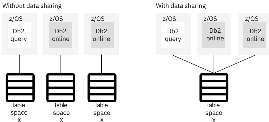
Figure 33. Flexible configurations with Db2 data sharing
