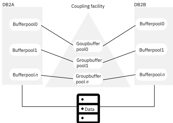
Figure 35. Relationship of buffer pools to group buffer pools
