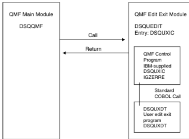
Figure 74. Program structure of a COBOL edit exit routine
