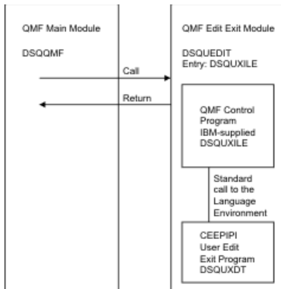
Figure 76. Program structure of a COBOL edit exit routine that uses the CEEPIPI interface
