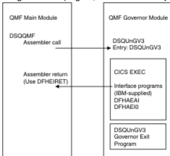
Figure 95. How QMF interacts with the governor exit in a CICS-supplied environment
