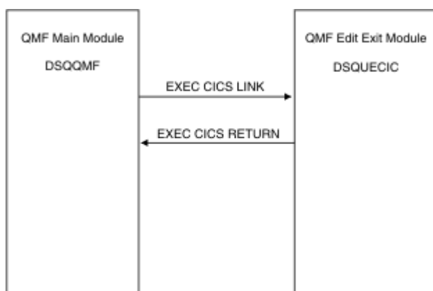
Figure 69. Program structure for PL/I edit exit routine in CICS
