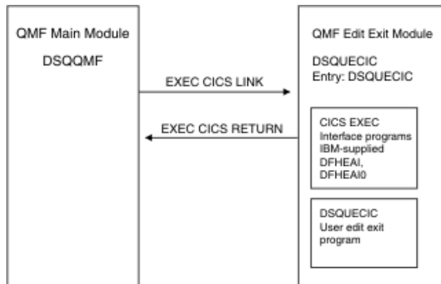
Figure 64. Program structure of an Assembler edit exit routine for CICS
