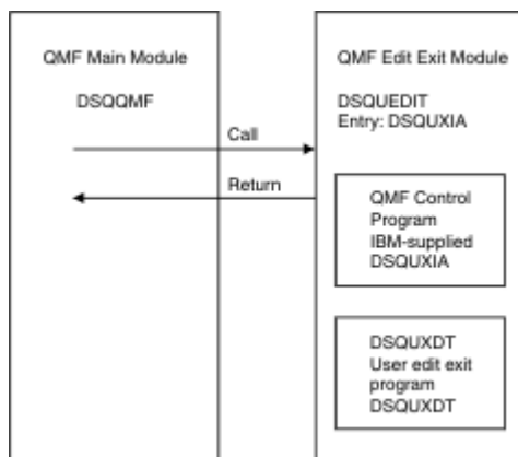
Figure 61. Program structure of an Assembler edit exit routine for TSO, ISPF, or native z/OS
