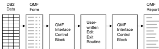
Figure 59. How a user edit routine works with QMF for TSO and CICS
