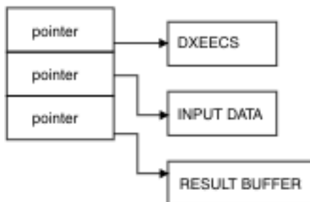
Figure 79. Providing addressability for your edit exit routine in CICS using the DFHCOMMAREA
