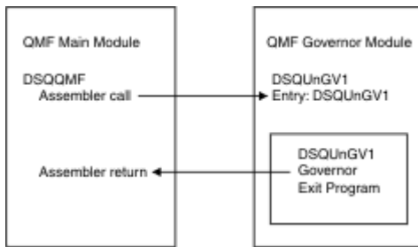
Figure 94. How QMF interacts with the governor exit under TSO, ISPF, or native z/OS
