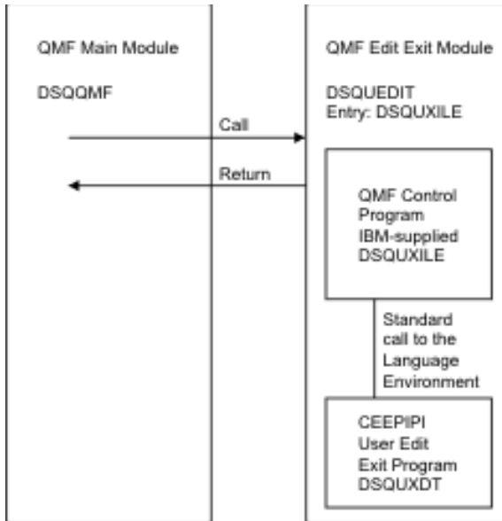
Figure 67. Program structure of a PL/I edit exit routine written with the CEEPIPI Language Environment interface
