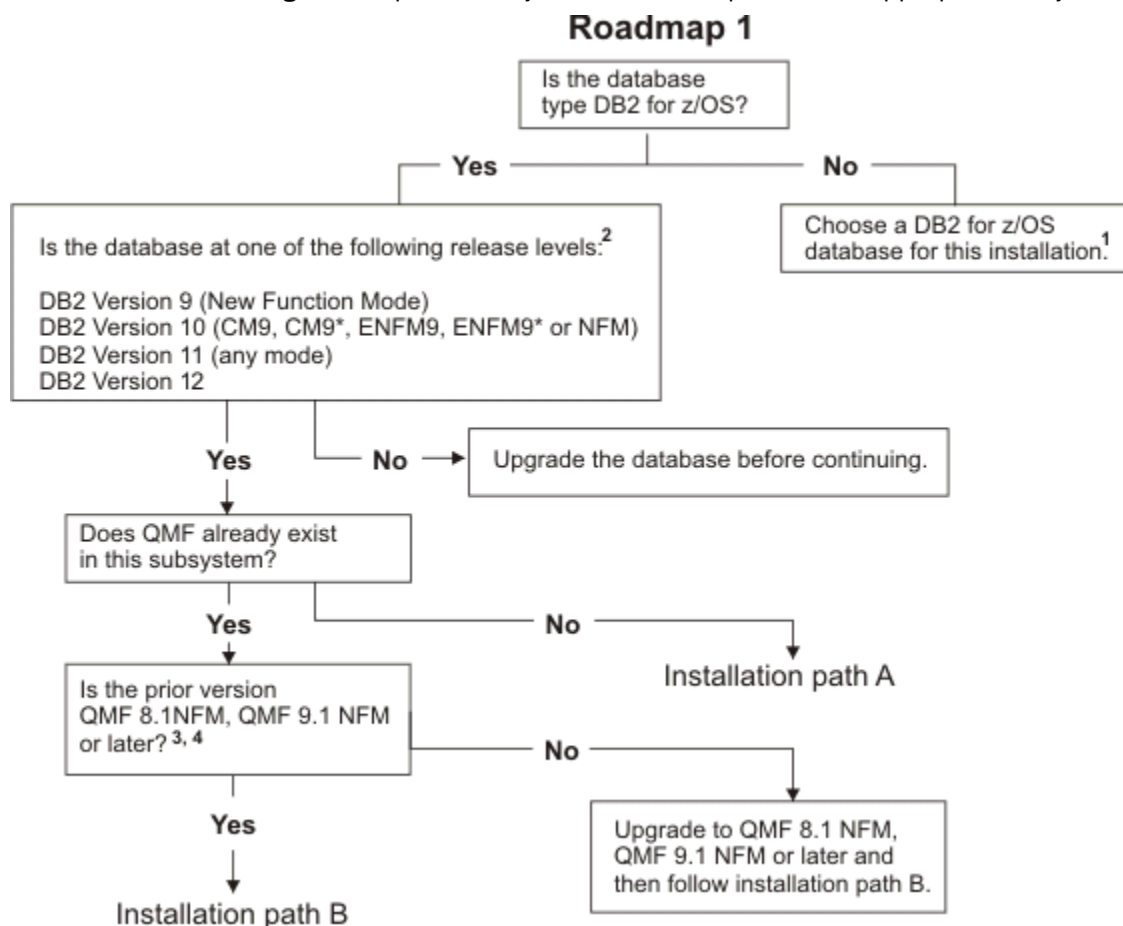
Figure 4. Installation roadmap for the first QMF Version 12 Release 2 installation or databases that will stand alone, function as requesters only, or function as both requesters and servers
