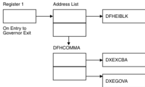
Figure 100. Contents of register 1 on a call to the governor exit routine in CICS
