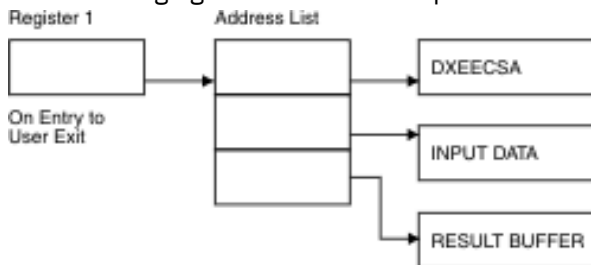
Figure 62. Conditions that exist on entry to the edit exit program in Assembler
