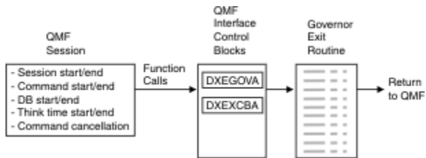
Figure 96. How a governor exit routine works with QMF for TSO and CICS
