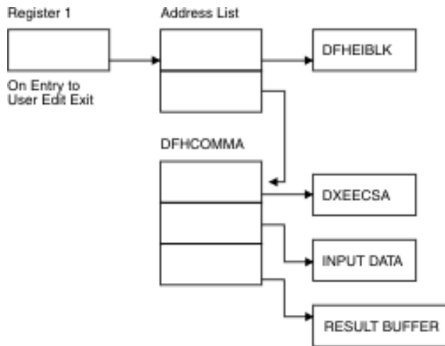
Figure 65. How a CICS Assembler edit routine interacts with QMF
