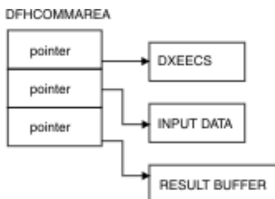
Figure 70. How DFHCOMMAREA, the CICS communications area, works
