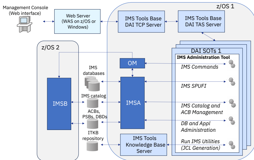
Figure 3. IMS Administration Tool functional architecture in multiple LPARs (Web client)
