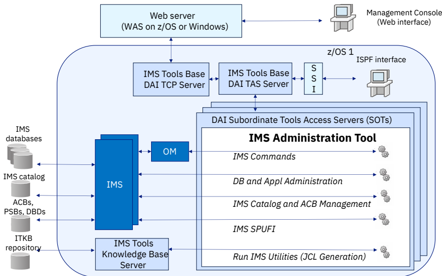
Figure 1. IMS Administration Tool functional architecture in a single LPAR
