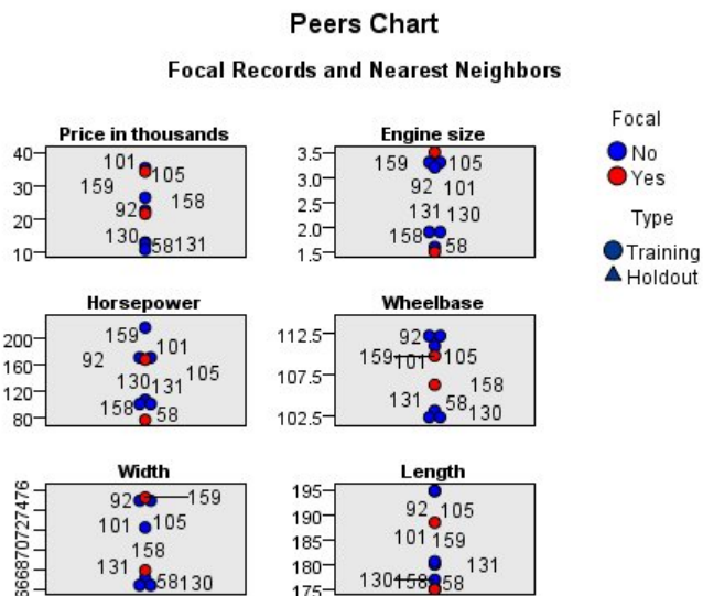
Figure 393. Peers chart
