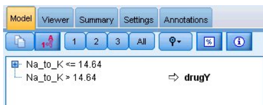
Figure 97. Rule browser
