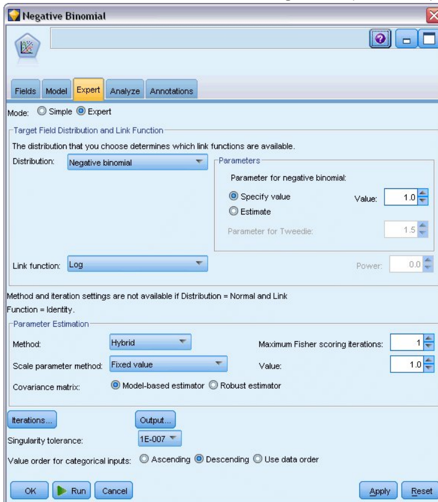
Figure 319. Expert tab
