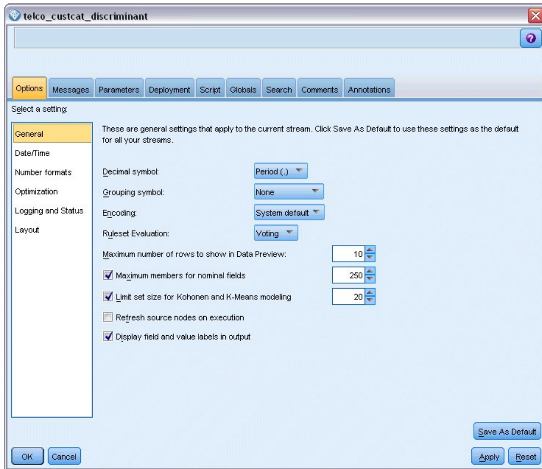
Figure 265. Stream properties
