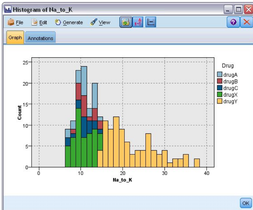
Figure 92. Histogram display
