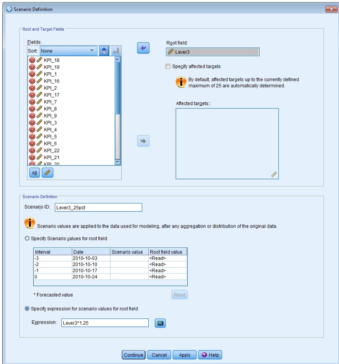
Figure 410. Scenario Definition
