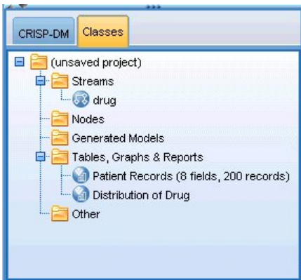
Figure 11. Classes view
