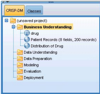
Figure 10. CRISP-DM view
