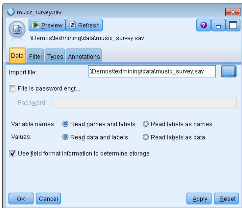
Figure 10. Statistics File node dialog box: Data tab
