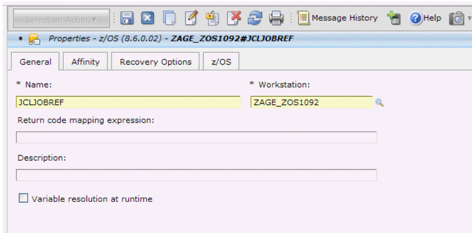
Figure 3. The General page of a new agent for z/OS definition
