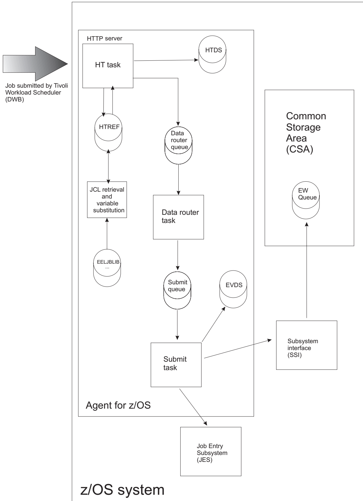
Figure 6. The route followed by a job within the agent for z/OS.
