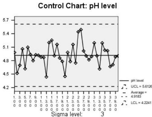
Figure 92. Individuals chart
