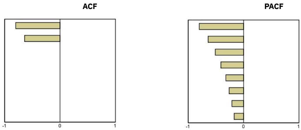
ARIMA(0,0,2), \rho_1 > 0
