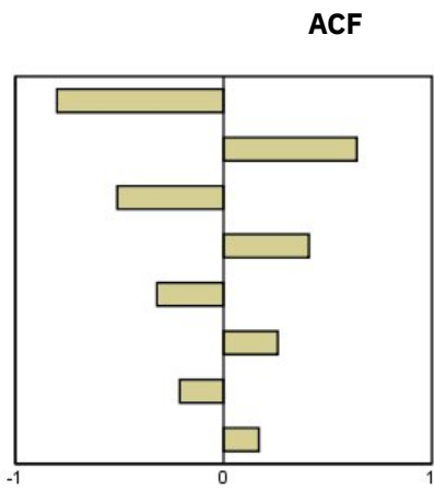
ARIMA(2,0,0), 1_2 > 0
