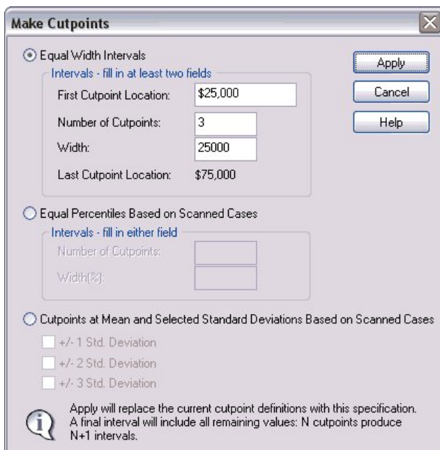
Figure 41. Make Cutpoints dialog box
