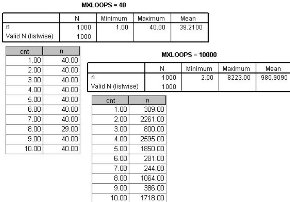
Figure 60. Different results with different MXLOOPS settings
