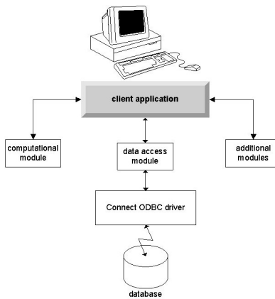
Figure 2. Connect ODBC in local analysis mode
