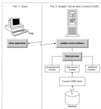
Figure 1. Connect ODBC in distributed analysis mode
