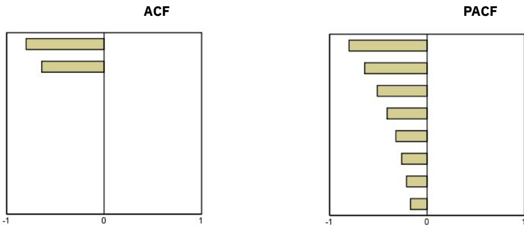
ARIMA(0,0,2), \alpha_1 \alpha_2 > 0
