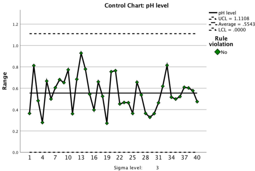
Figure 89. R chart
