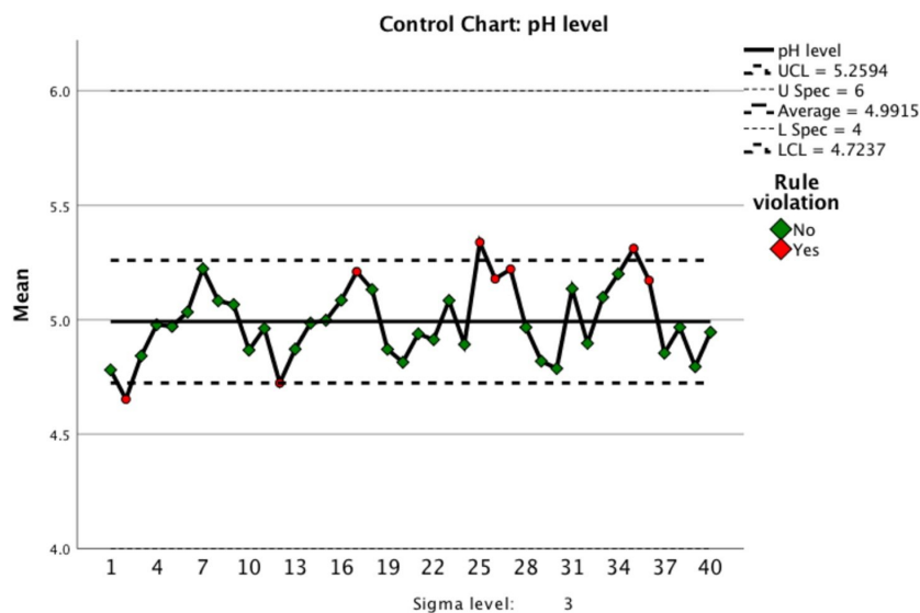
Figure 88. X-bar chart
