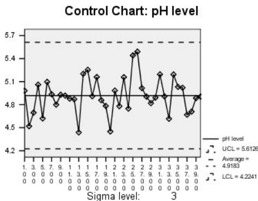
Figure 91. Individuals chart
