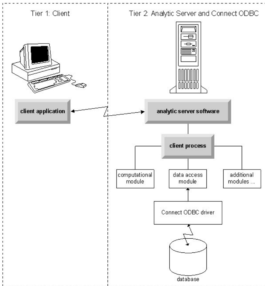
Figure 1. Connect ODBC in distributed analysis mode
