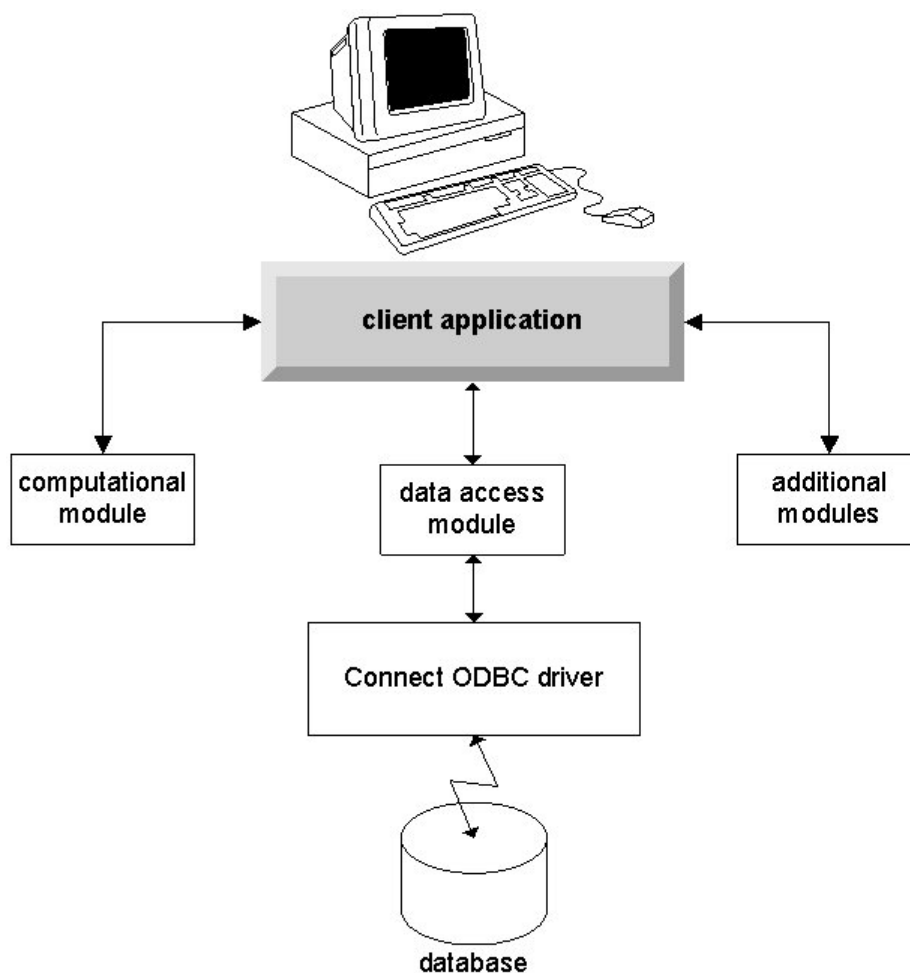
Figure 2. Connect ODBC in local analysis mode
