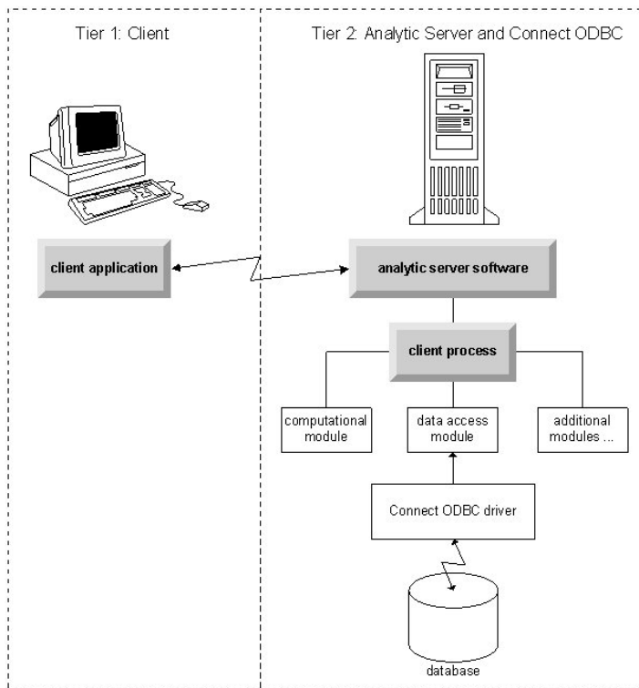
Figure 3. Connect ODBC in distributed analysis mode
