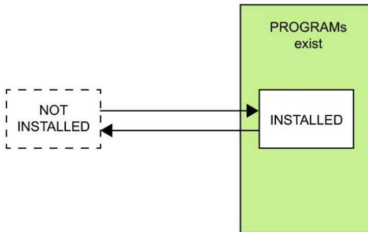
Figure 3. The lifecycle of a stand-alone web application, showing when PROGRAM resources for @CICSPprogram annotations exist
