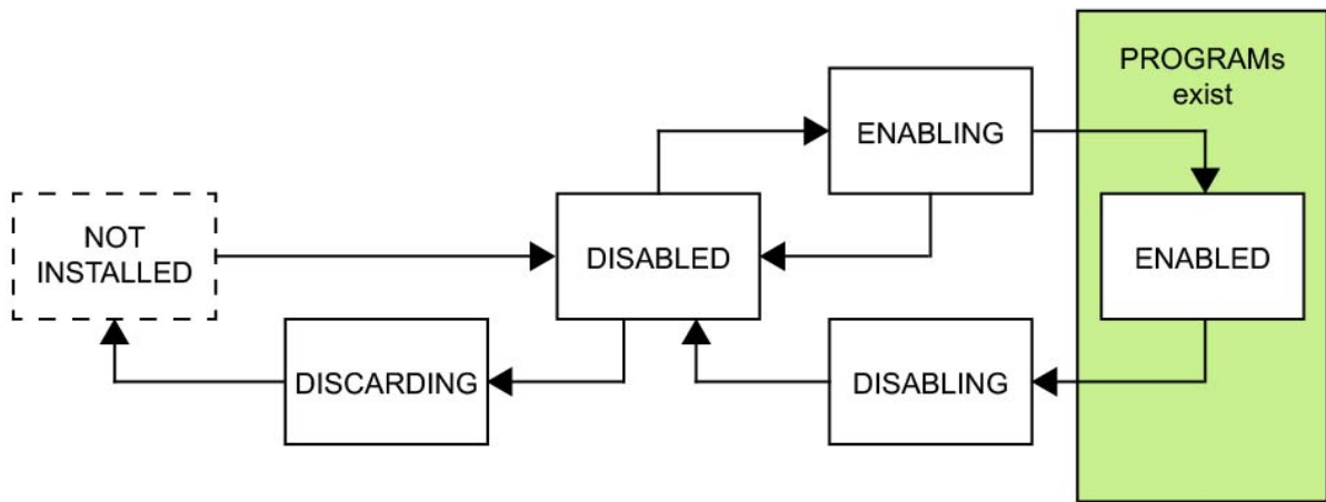
Figure 2. The lifecycle of a CICS bundle, showing when PROGRAM resources for @CICSPprogram annotations exist
