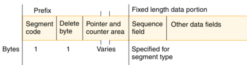
Figure 9. Format of fixed-length segments
