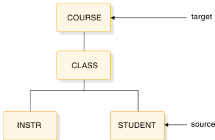
Figure 186. Database record showing the source and target for secondary indexes
