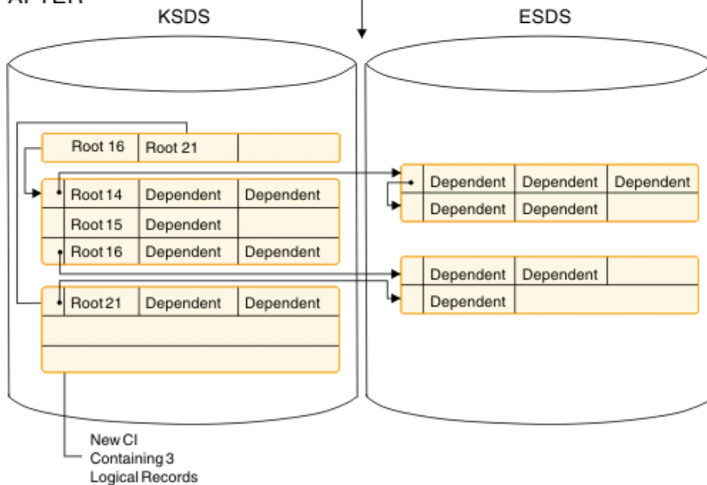
Figure 28. Inserting a root segment into a HISAM database (no free logical record exists in the CI)
