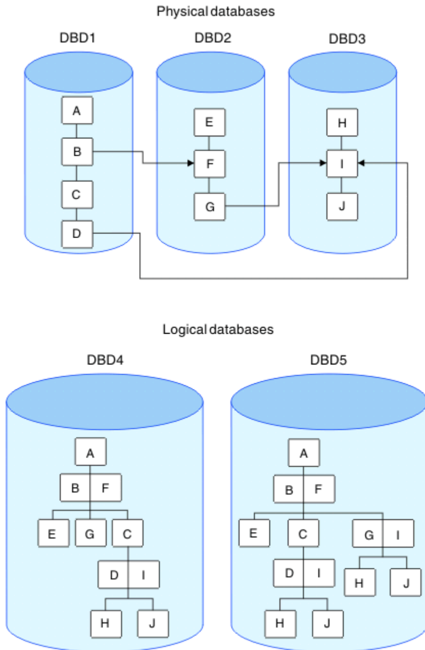
Figure 97. The first logical relationship crossed in a hierarchical path of a logical database
