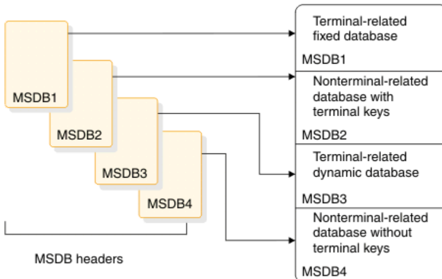
Figure 66. MSDB pointers
