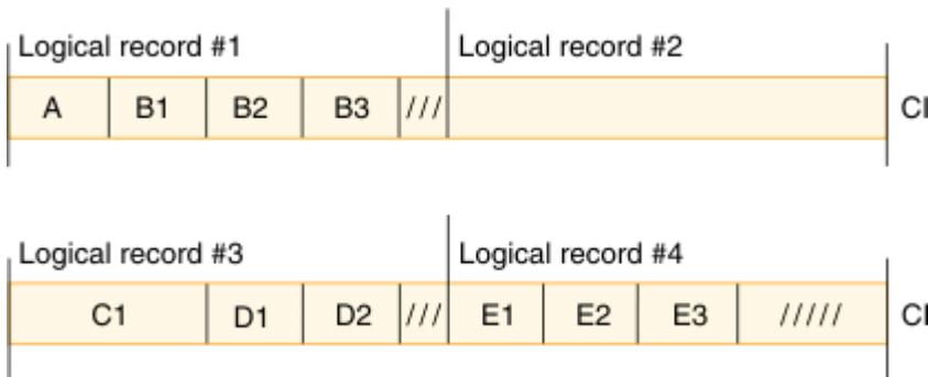
Figure 227. Logical records example with two read operations
