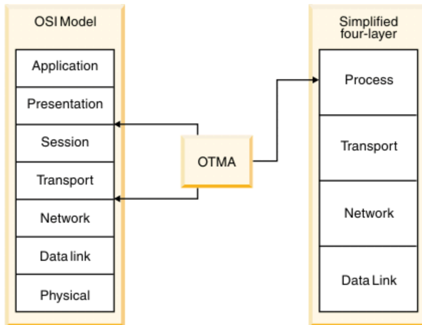
Figure 127. Network architecture models
