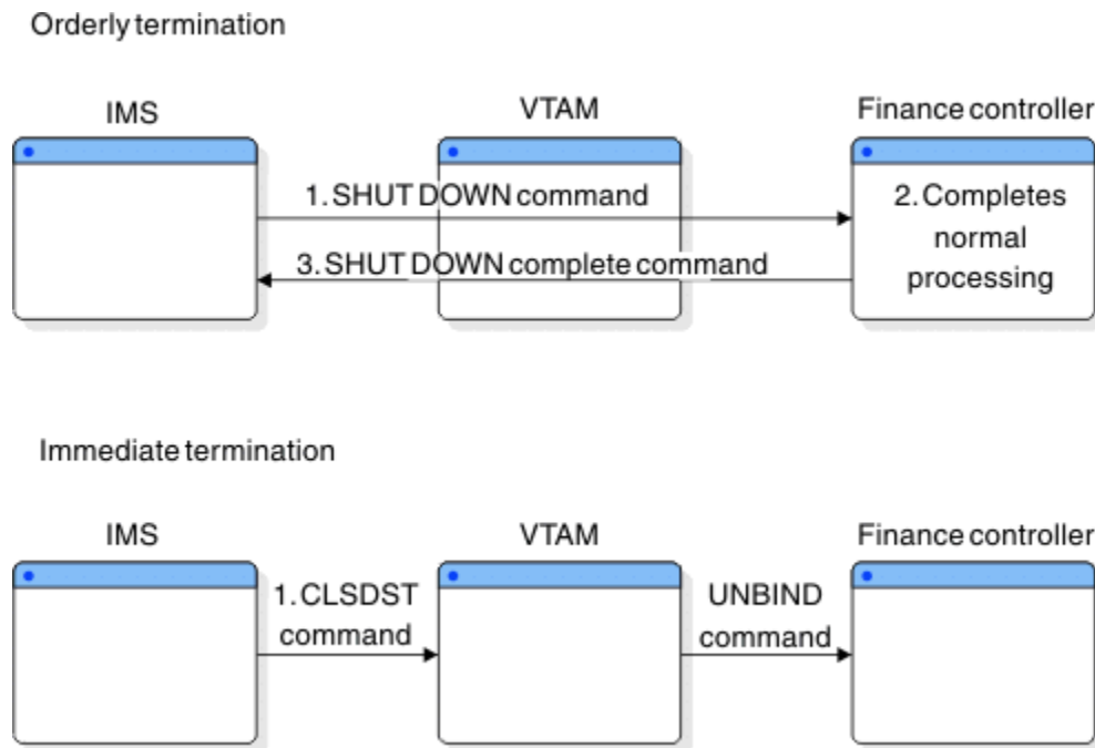
Figure 157. Termination processing
